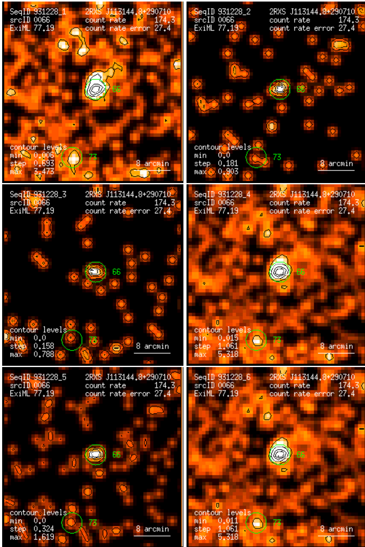
Figure 66: RASS 931228: detection 0066: band rate images, Gaussian filter: (1) PSPC channels 11 – 41, (2) 52 – 90, (3) 91 – 201, (4) 11 – 235, (5) 52 – 201, (6) 11 – 201. Broad band rates in counts/ks. Band rate contour levels in counts/ks/arcmin 2 .
