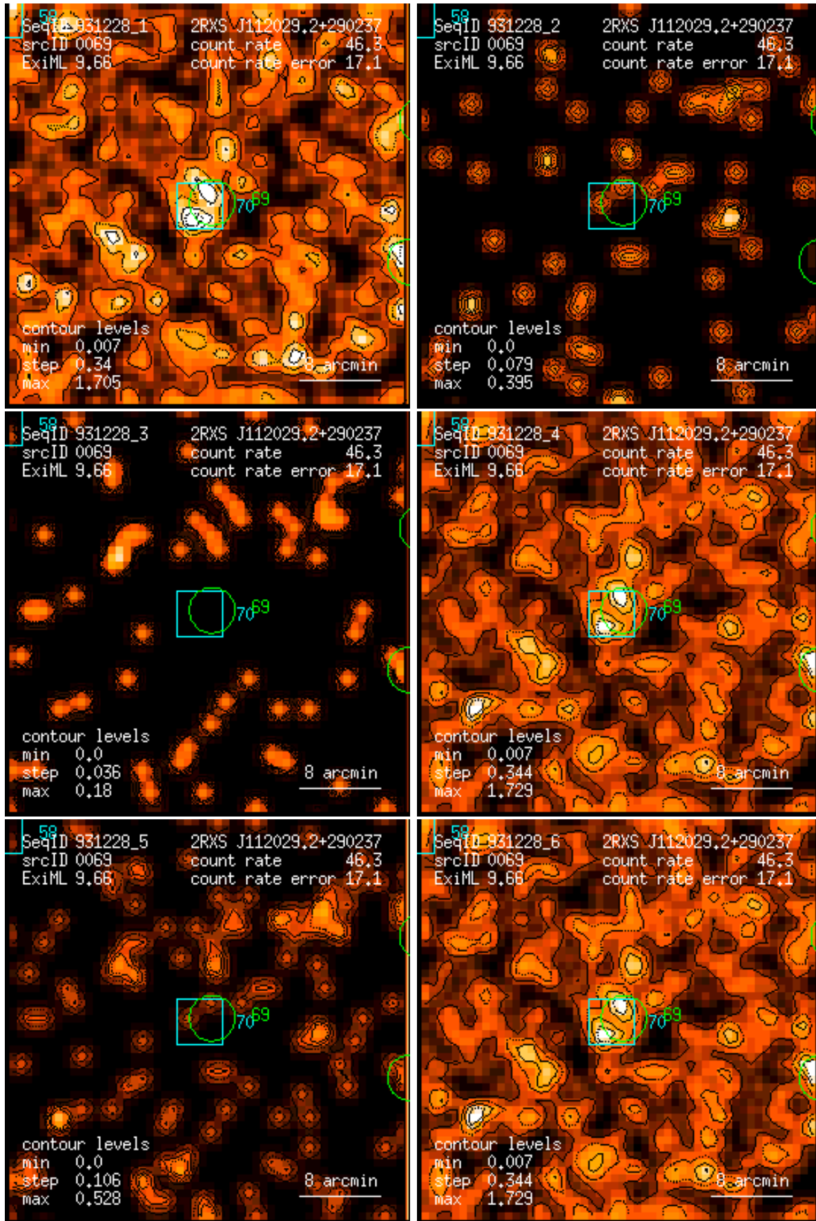
Figure 69: RASS 931228: detection 0069: band rate images, Gaussian filter: (1) PSPC channels 11 – 41, (2) 52 – 90, (3) 91 – 201, (4) 11 – 235, (5) 52 – 201, (6) 11 – 201. Broad band rates in counts/ks. Band rate contour levels in counts/ks/arcmin 2 .
