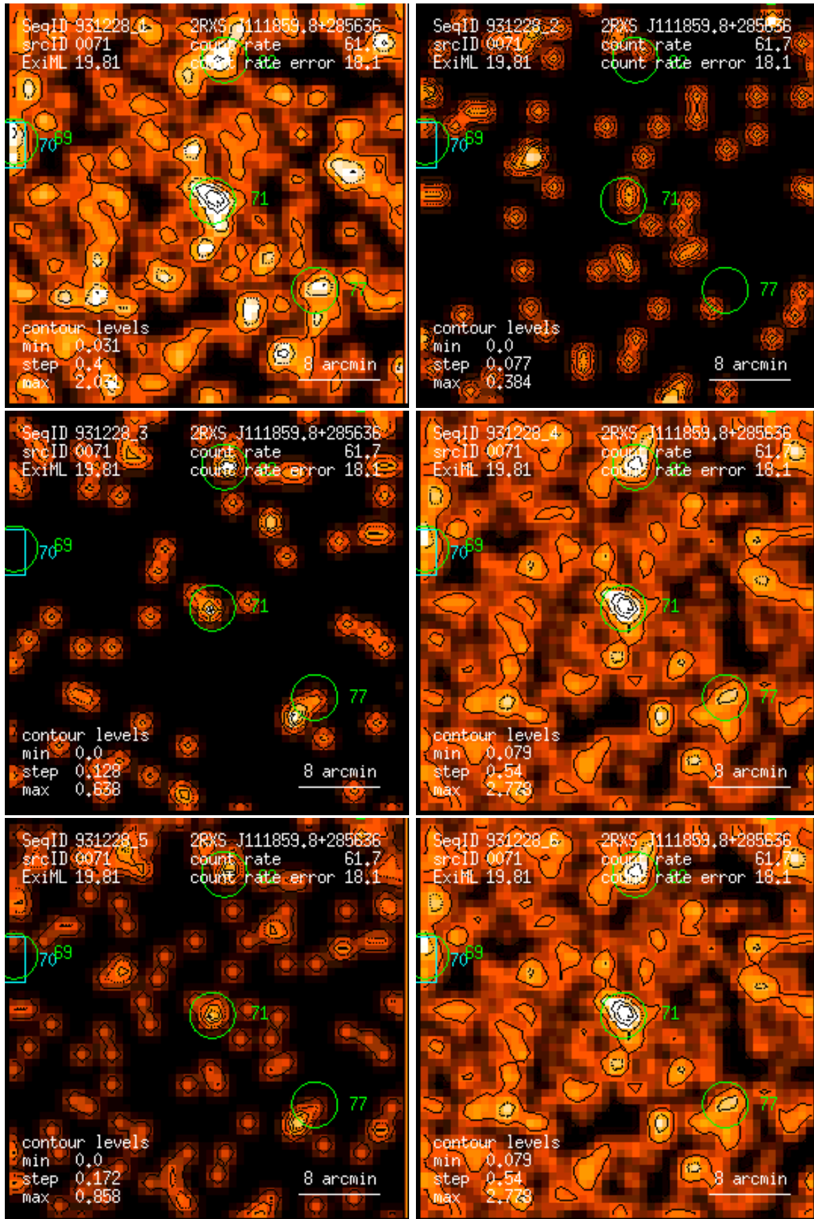
Figure 71: RASS 931228: detection 0071: band rate images, Gaussian filter: (1) PSPC channels 11 – 41, (2) 52 – 90, (3) 91 – 201, (4) 11 – 235, (5) 52 – 201, (6) 11 – 201. Broad band rates in counts/ks. Band rate contour levels in counts/ks/arcmin 2 .
