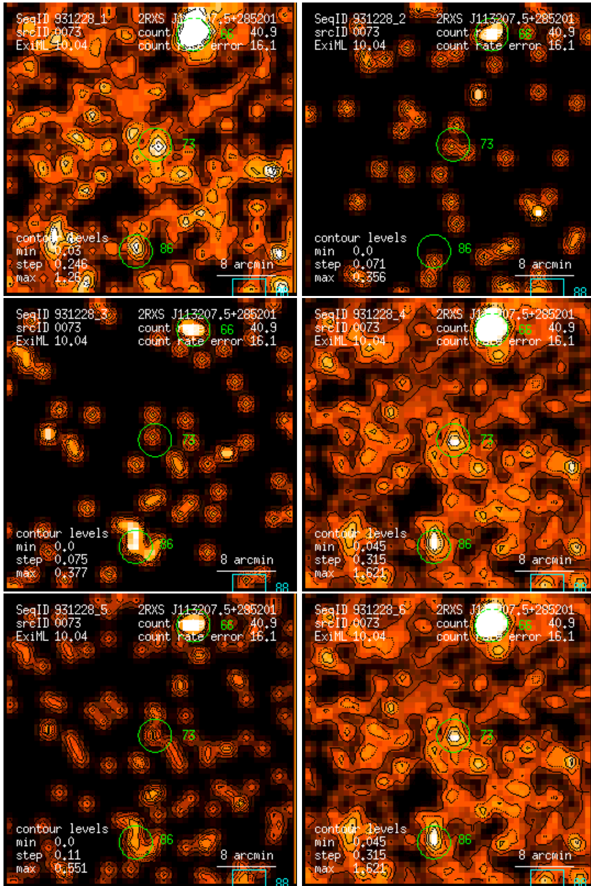
Figure 73: RASS 931228: detection 0073: band rate images, Gaussian filter: (1) PSPC channels 11 – 41, (2) 52 – 90, (3) 91 – 201, (4) 11 – 235, (5) 52 – 201, (6) 11 – 201. Broad band rates in counts/ks. Band rate contour levels in counts/ks/arcmin 2 .
