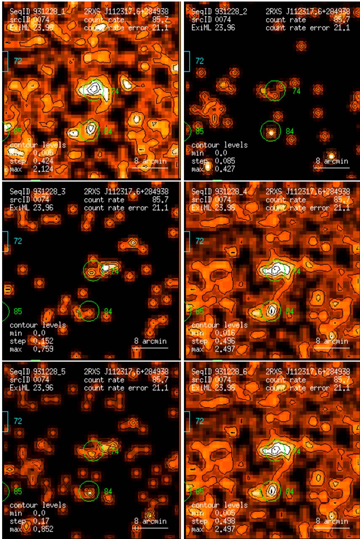
Figure 74: RASS 931228: detection 0074: band rate images, Gaussian filter: (1) PSPC channels 11 – 41, (2) 52 – 90, (3) 91 – 201, (4) 11 – 235, (5) 52 – 201, (6) 11 – 201. Broad band rates in counts/ks. Band rate contour levels in counts/ks/arcmin 2 .
