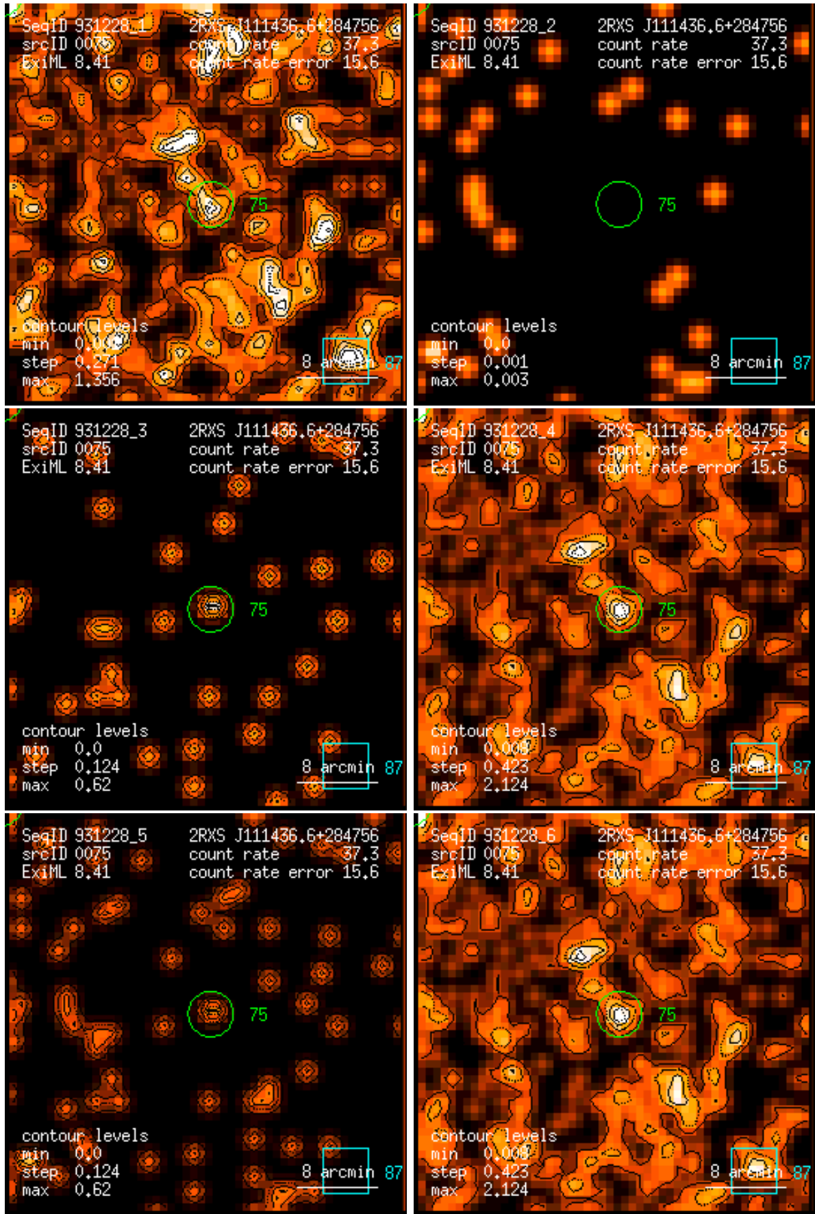
Figure 75: RASS 931228: detection 0075: band rate images, Gaussian filter: (1) PSPC channels 11 – 41, (2) 52 – 90, (3) 91 – 201, (4) 11 – 235, (5) 52 – 201, (6) 11 – 201. Broad band rates in counts/ks. Band rate contour levels in counts/ks/arcmin 2 .
