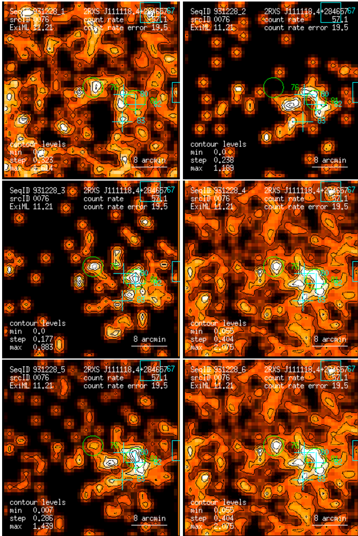
Figure 76: RASS 931228: detection 0076: band rate images, Gaussian filter: (1) PSPC channels 11 – 41, (2) 52 – 90, (3) 91 – 201, (4) 11 – 235, (5) 52 – 201, (6) 11 – 201. Broad band rates in counts/ks. Band rate contour levels in counts/ks/arcmin 2 .
