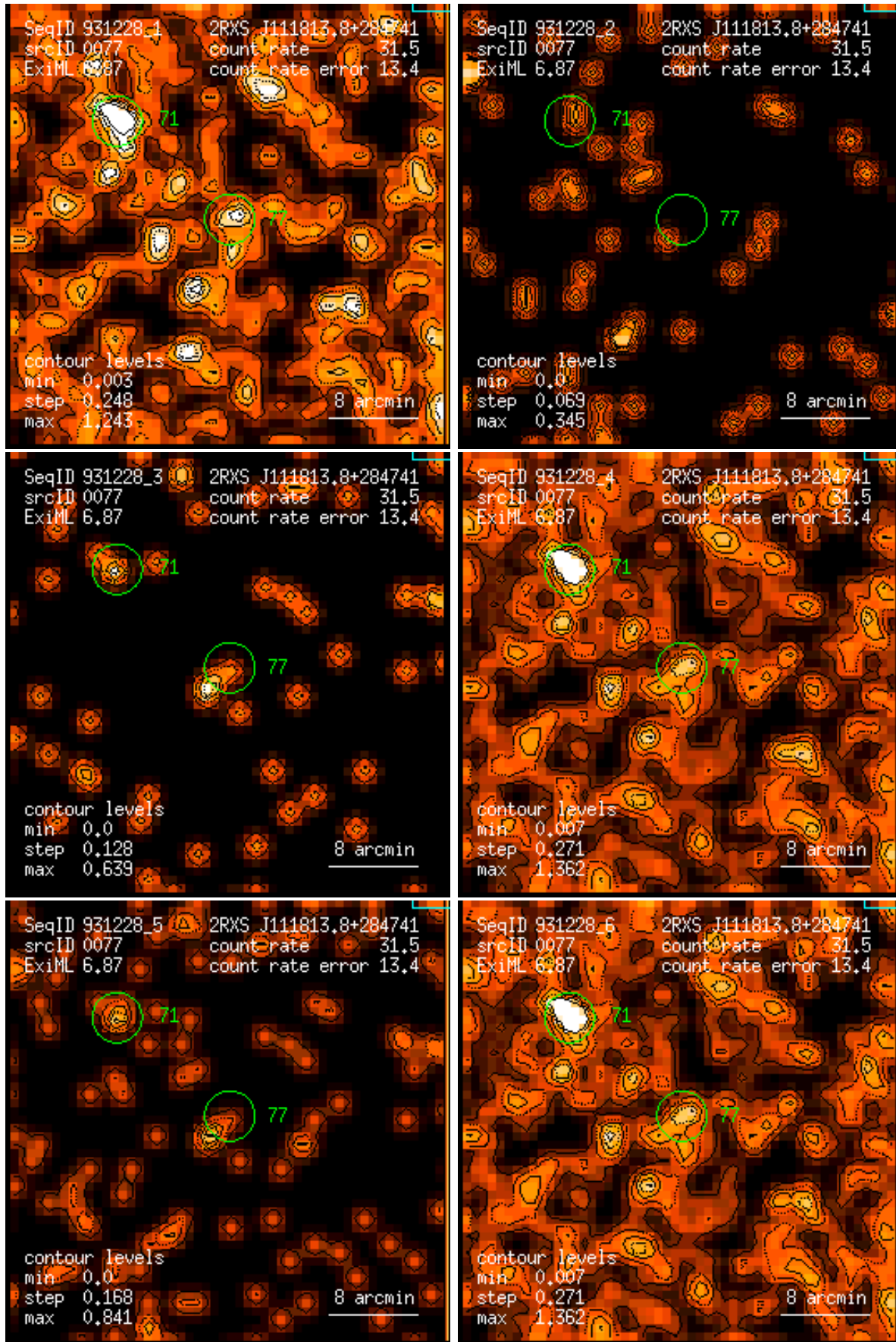
Figure 77: RASS 931228: detection 0077: band rate images, Gaussian filter: (1) PSPC channels 11 – 41, (2) 52 – 90, (3) 91 – 201, (4) 11 – 235, (5) 52 – 201, (6) 11 – 201. Broad band rates in counts/ks. Band rate contour levels in counts/ks/arcmin 2 .
