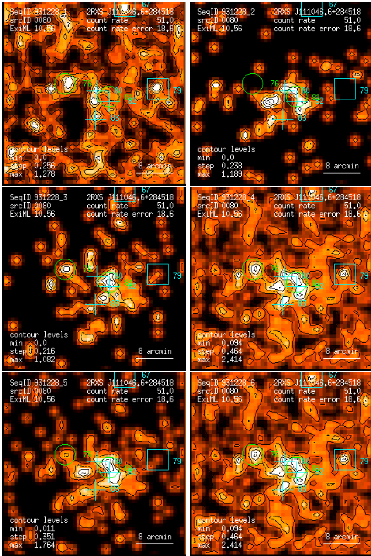
Figure 80: RASS 931228: detection 0080: band rate images, Gaussian filter: (1) PSPC channels 11 – 41, (2) 52 – 90, (3) 91 – 201, (4) 11 – 235, (5) 52 – 201, (6) 11 – 201. Broad band rates in counts/ks. Band rate contour levels in counts/ks/arcmin 2 .
