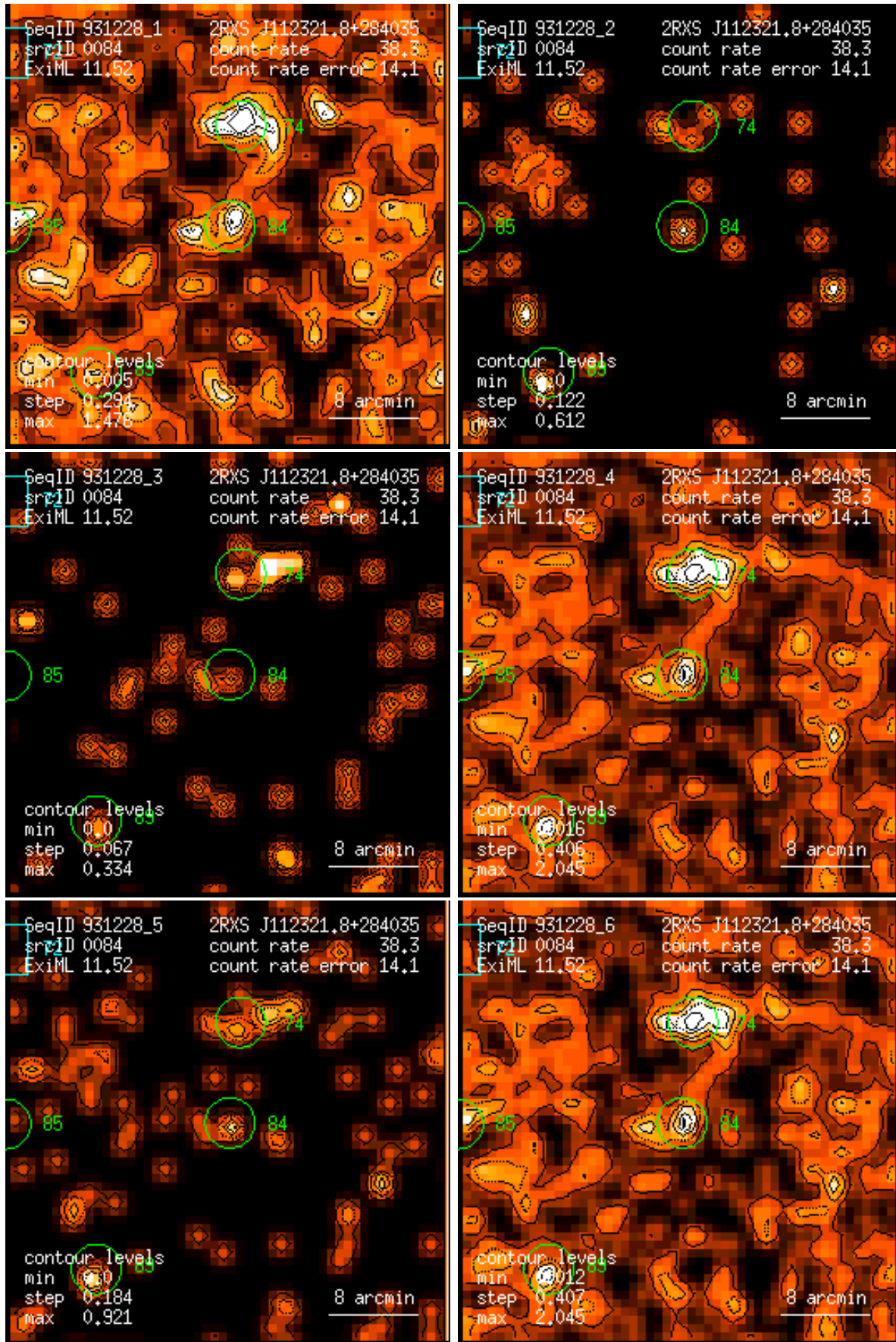
Figure 84: RASS 931228: detection 0084: band rate images, Gaussian filter: (1) PSPC channels 11 – 41, (2) 52 – 90, (3) 91 – 201, (4) 11 – 235, (5) 52 – 201, (6) 11 – 201. Broad band rates in counts/ks. Band rate contour levels in counts/ks/arcmin 2 .
