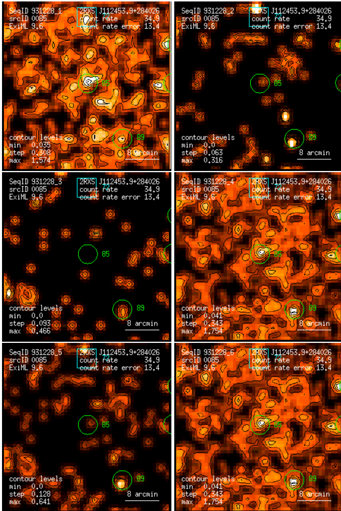
Figure 85: RASS 931228: detection 0085: band rate images, Gaussian filter: (1) PSPC channels 11 – 41, (2) 52 – 90, (3) 91 – 201, (4) 11 – 235, (5) 52 – 201, (6) 11 – 201. Broad band rates in counts/ks. Band rate contour levels in counts/ks/arcmin 2 .
