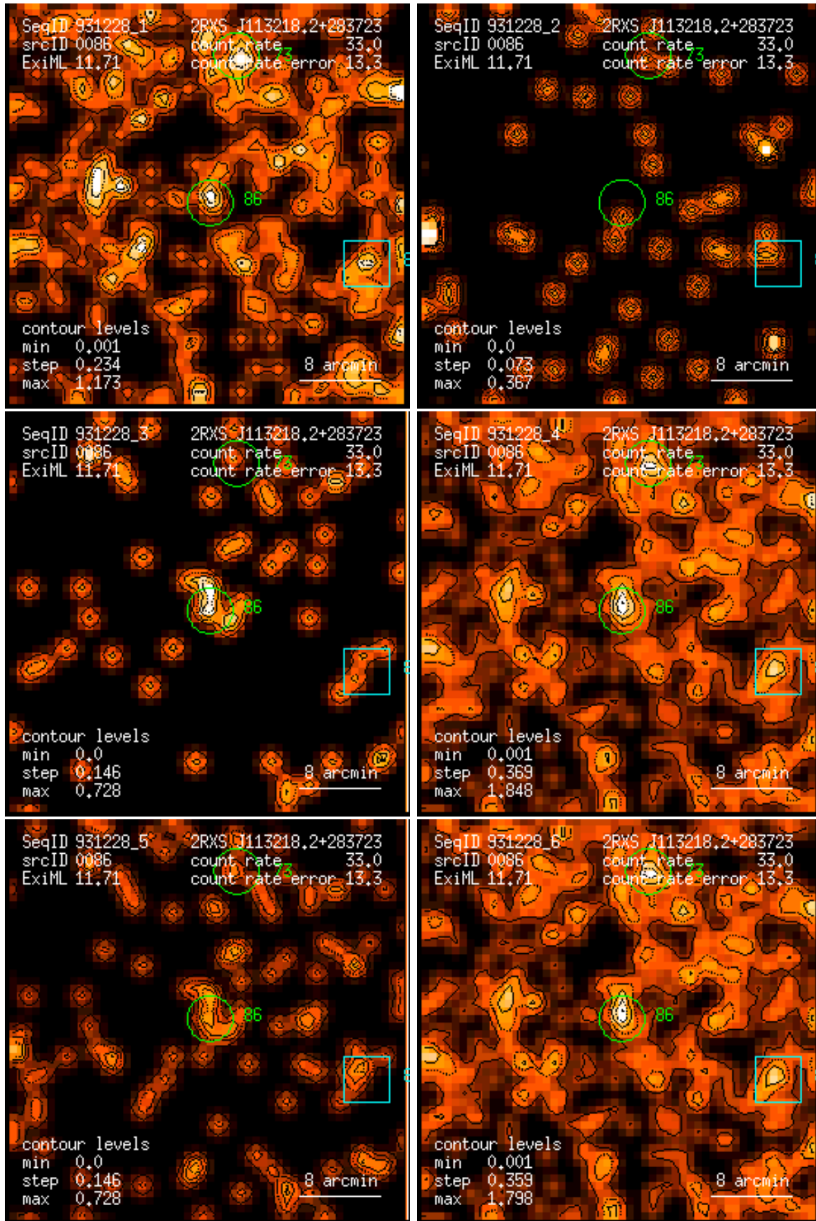
Figure 86: RASS 931228: detection 0086: band rate images, Gaussian filter: (1) PSPC channels 11 – 41, (2) 52 – 90, (3) 91 – 201, (4) 11 – 235, (5) 52 – 201, (6) 11 – 201. Broad band rates in counts/ks. Band rate contour levels in counts/ks/arcmin 2 .
