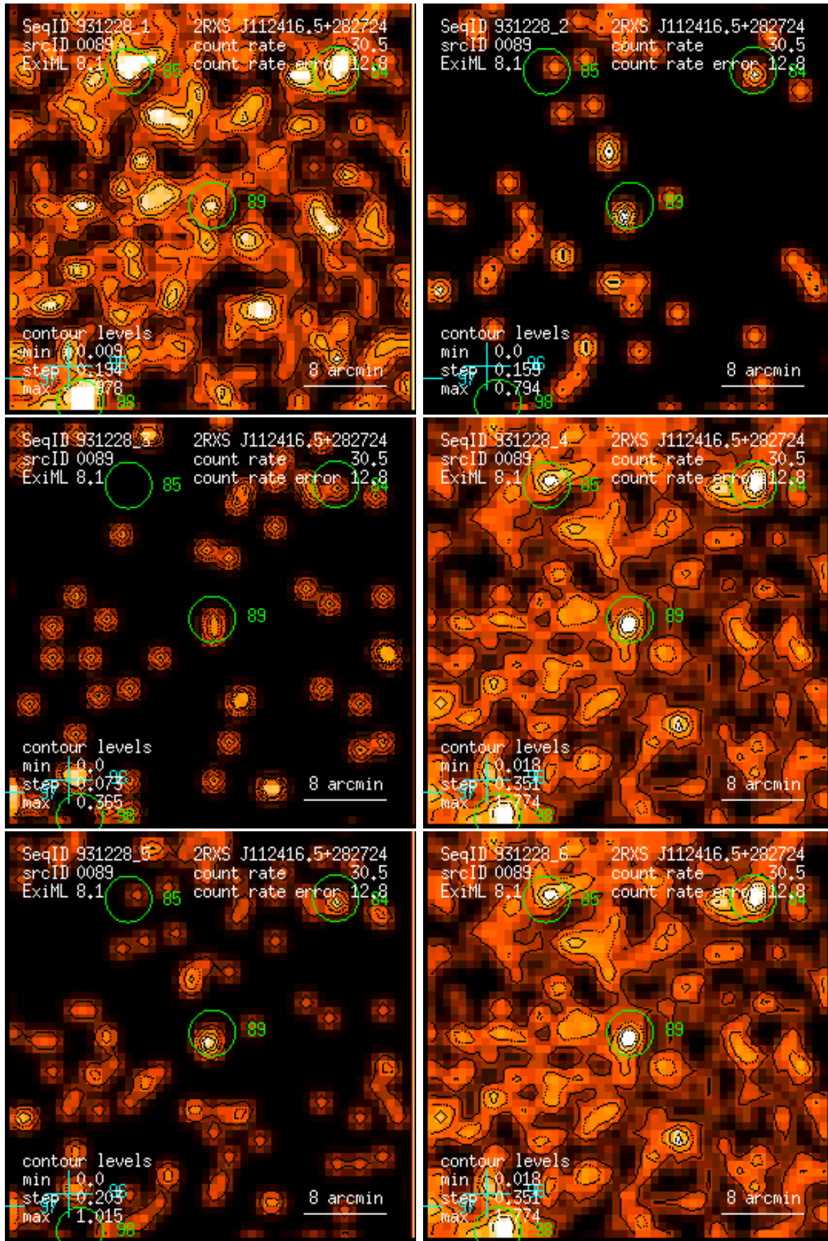
Figure 89: RASS 931228: detection 0089: band rate images, Gaussian filter: (1) PSPC channels 11 – 41, (2) 52 – 90, (3) 91 – 201, (4) 11 – 235, (5) 52 – 201, (6) 11 – 201. Broad band rates in counts/ks. Band rate contour levels in counts/ks/arcmin 2 .
