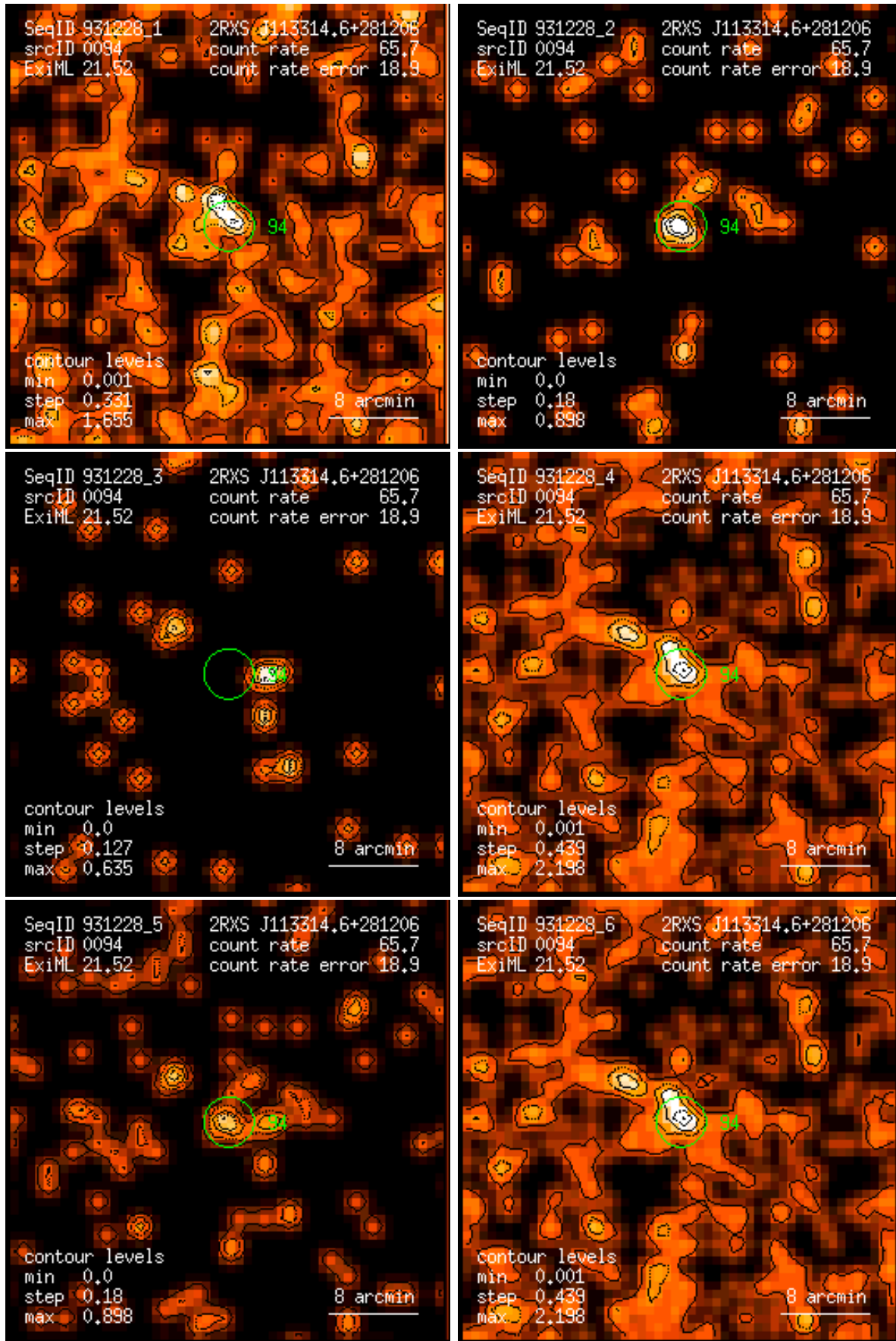
Figure 94: RASS 931228: detection 0094: band rate images, Gaussian filter: (1) PSPC channels 11 – 41, (2) 52 – 90, (3) 91 – 201, (4) 11 – 235, (5) 52 – 201, (6) 11 – 201. Broad band rates in counts/ks. Band rate contour levels in counts/ks/arcmin 2 .
