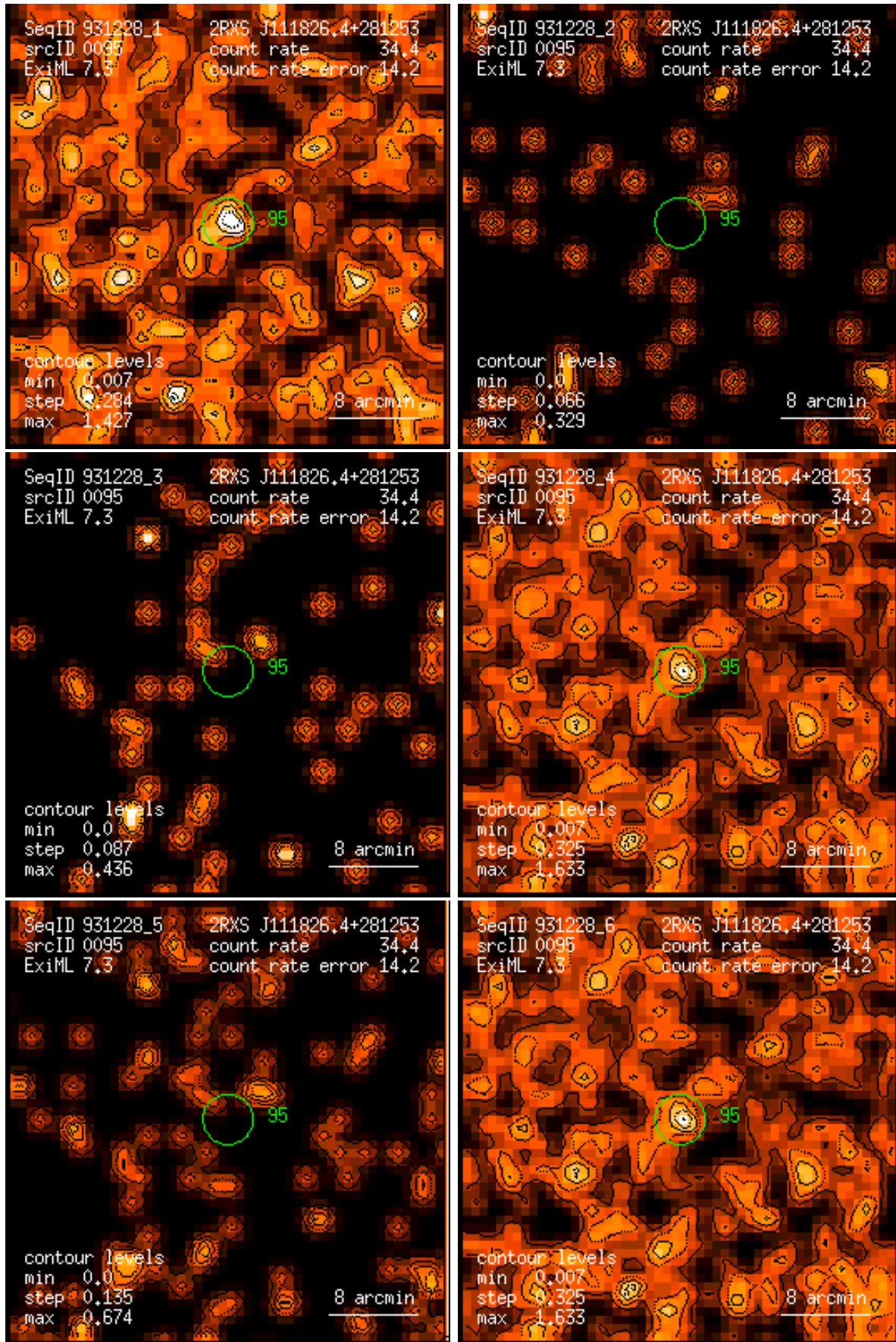
Figure 95: RASS 931228: detection 0095: band rate images, Gaussian filter: (1) PSPC channels 11 – 41, (2) 52 – 90, (3) 91 – 201, (4) 11 – 235, (5) 52 – 201, (6) 11 – 201. Broad band rates in counts/ks. Band rate contour levels in counts/ks/arcmin 2 .
