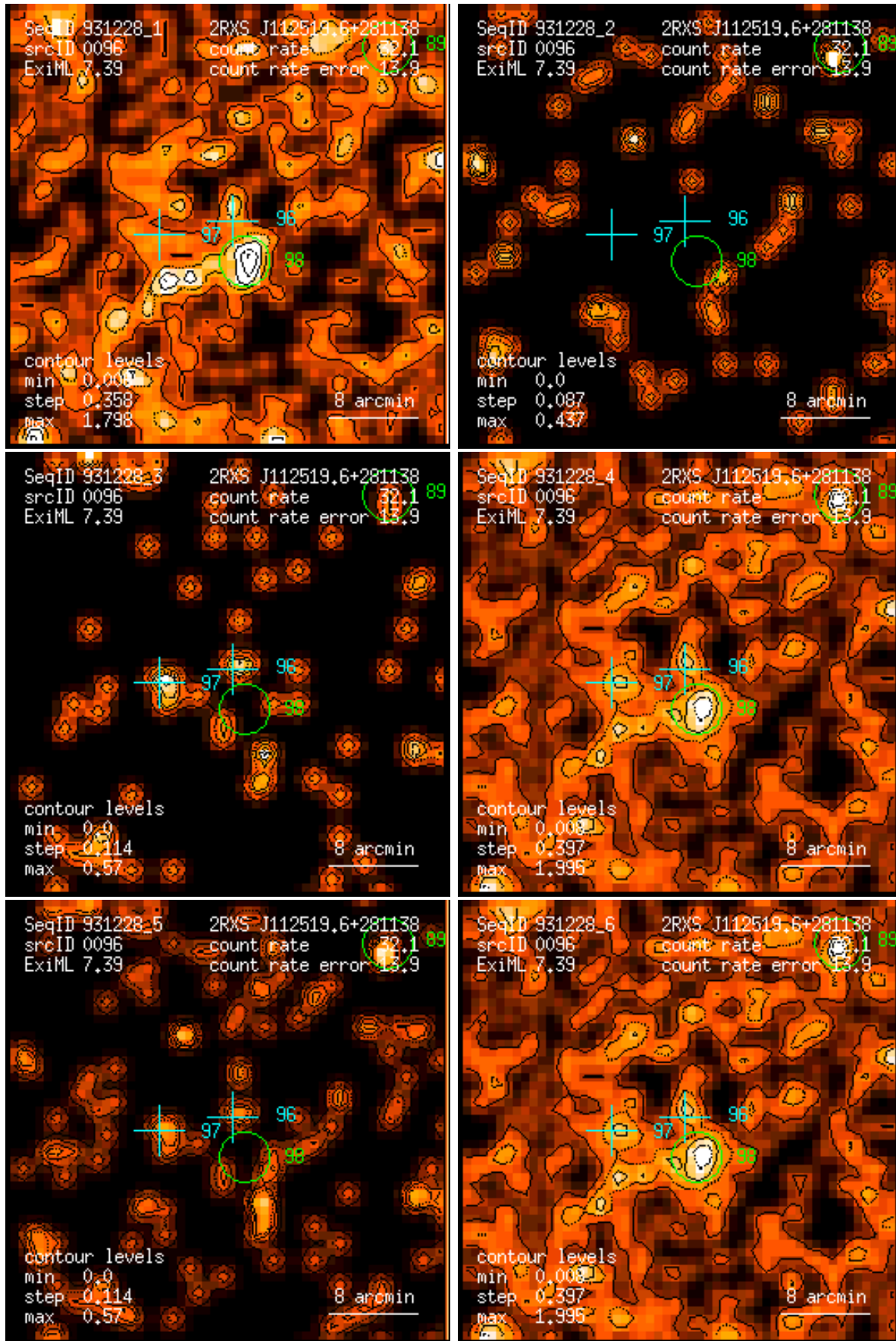
Figure 96: RASS 931228: detection 0096: band rate images, Gaussian filter: (1) PSPC channels 11 – 41, (2) 52 – 90, (3) 91 – 201, (4) 11 – 235, (5) 52 – 201, (6) 11 – 201. Broad band rates in counts/ks. Band rate contour levels in counts/ks/arcmin 2 .
