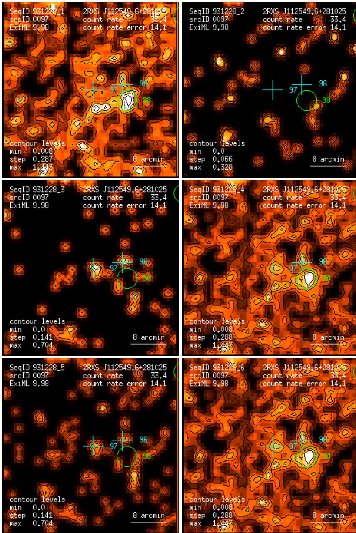
Figure 97: RASS 931228: detection 0097: band rate images, Gaussian filter: (1) PSPC channels 11 – 41, (2) 52 – 90, (3) 91 – 201, (4) 11 – 235, (5) 52 – 201, (6) 11 – 201. Broad band rates in counts/ks. Band rate contour levels in counts/ks/arcmin 2 .
