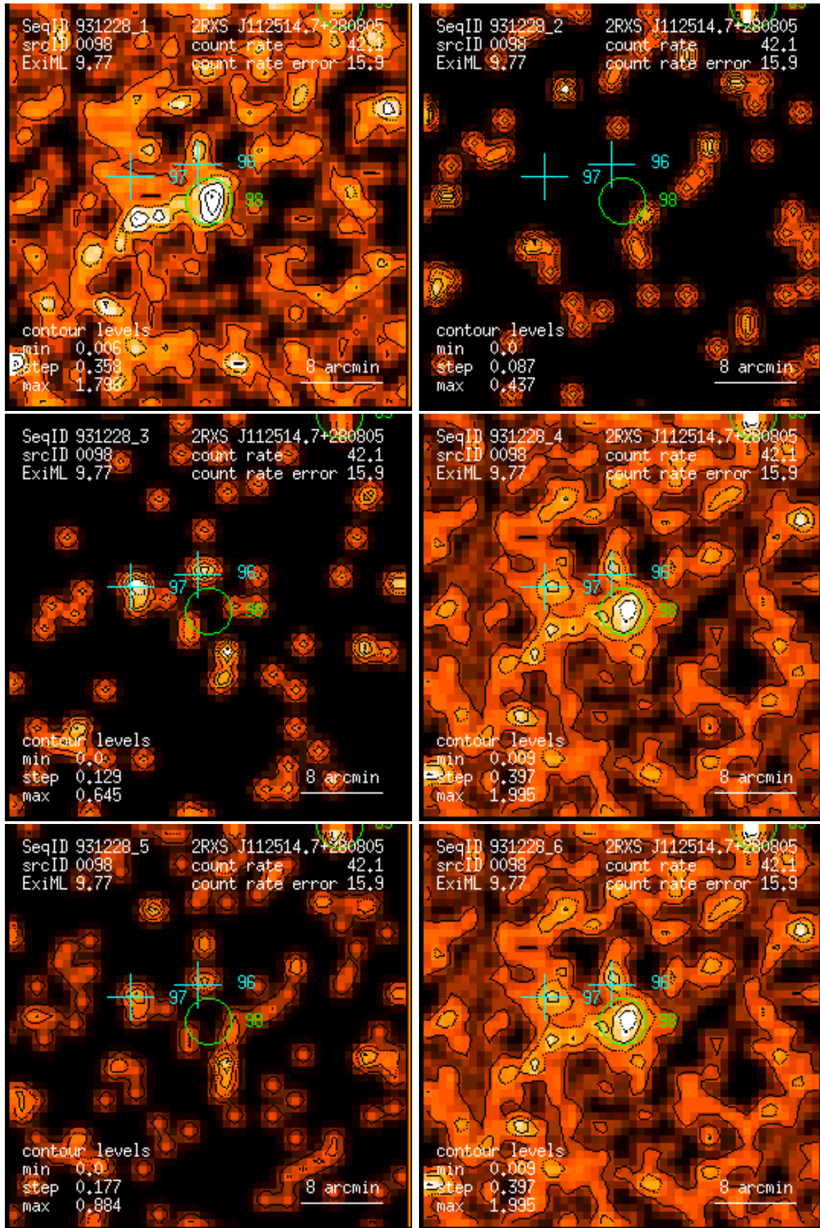
Figure 98: RASS 931228: detection 0098: band rate images, Gaussian filter: (1) PSPC channels 11 – 41, (2) 52 – 90, (3) 91 – 201, (4) 11 – 235, (5) 52 – 201, (6) 11 – 201. Broad band rates in counts/ks. Band rate contour levels in counts/ks/arcmin 2 .
