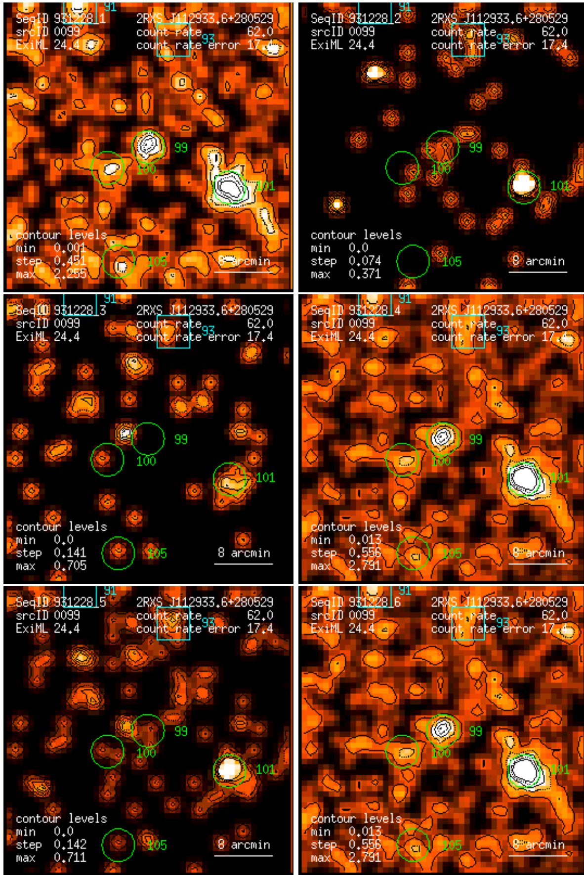
Figure 99: RASS 931228: detection 0099: band rate images, Gaussian filter: (1) PSPC channels 11 – 41, (2) 52 – 90, (3) 91 – 201, (4) 11 – 235, (5) 52 – 201, (6) 11 – 201. Broad band rates in counts/ks. Band rate contour levels in counts/ks/arcmin 2 .
