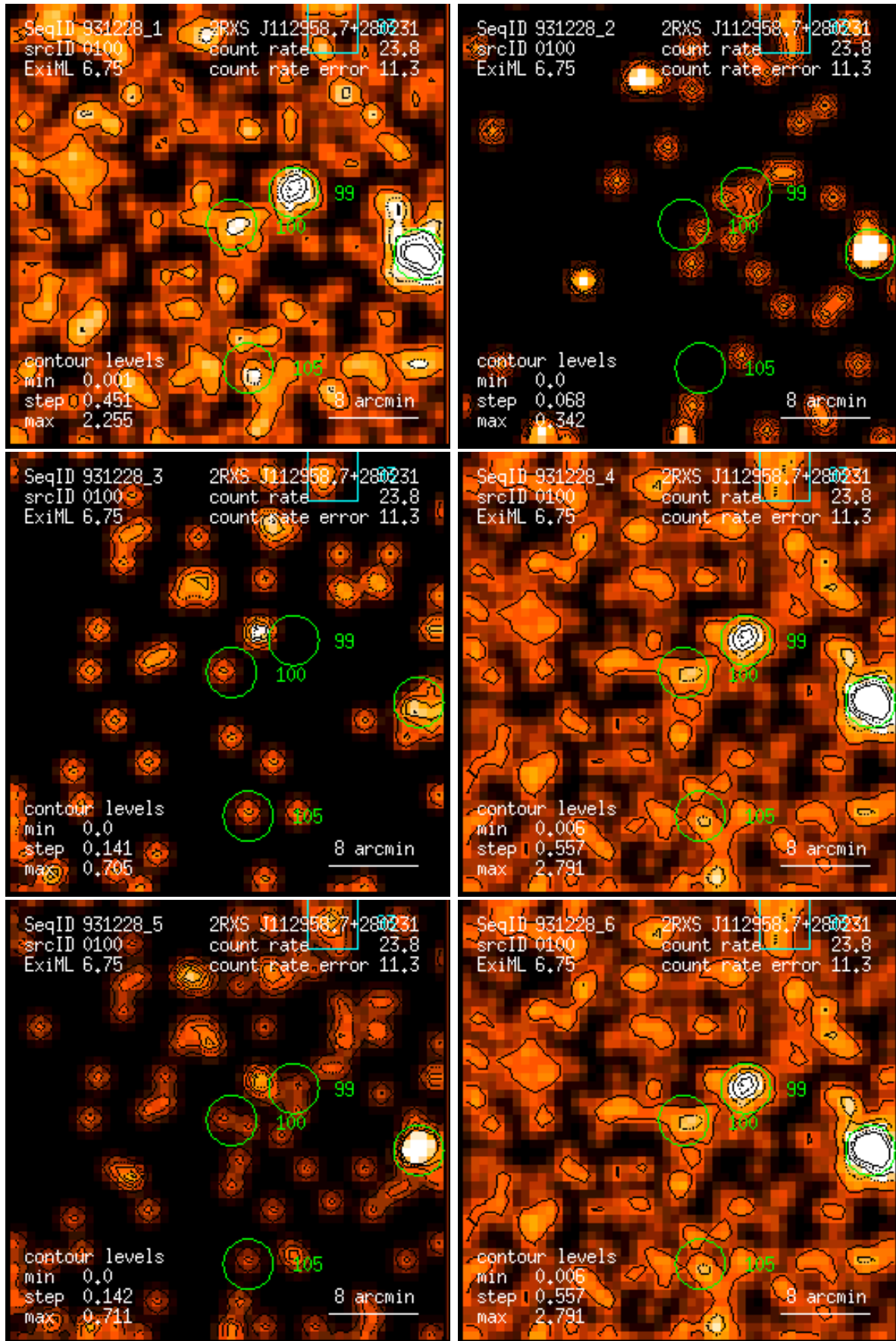
Figure 100: RASS 931228: detection 0100: band rate images, Gaussian filter: (1) PSPC channels 11 – 41, (2) 52 – 90, (3) 91 – 201, (4) 11 – 235, (5) 52 – 201, (6) 11 – 201. Broad band rates in counts/ks. Band rate contour levels in counts/ks/arcmin 2 .
