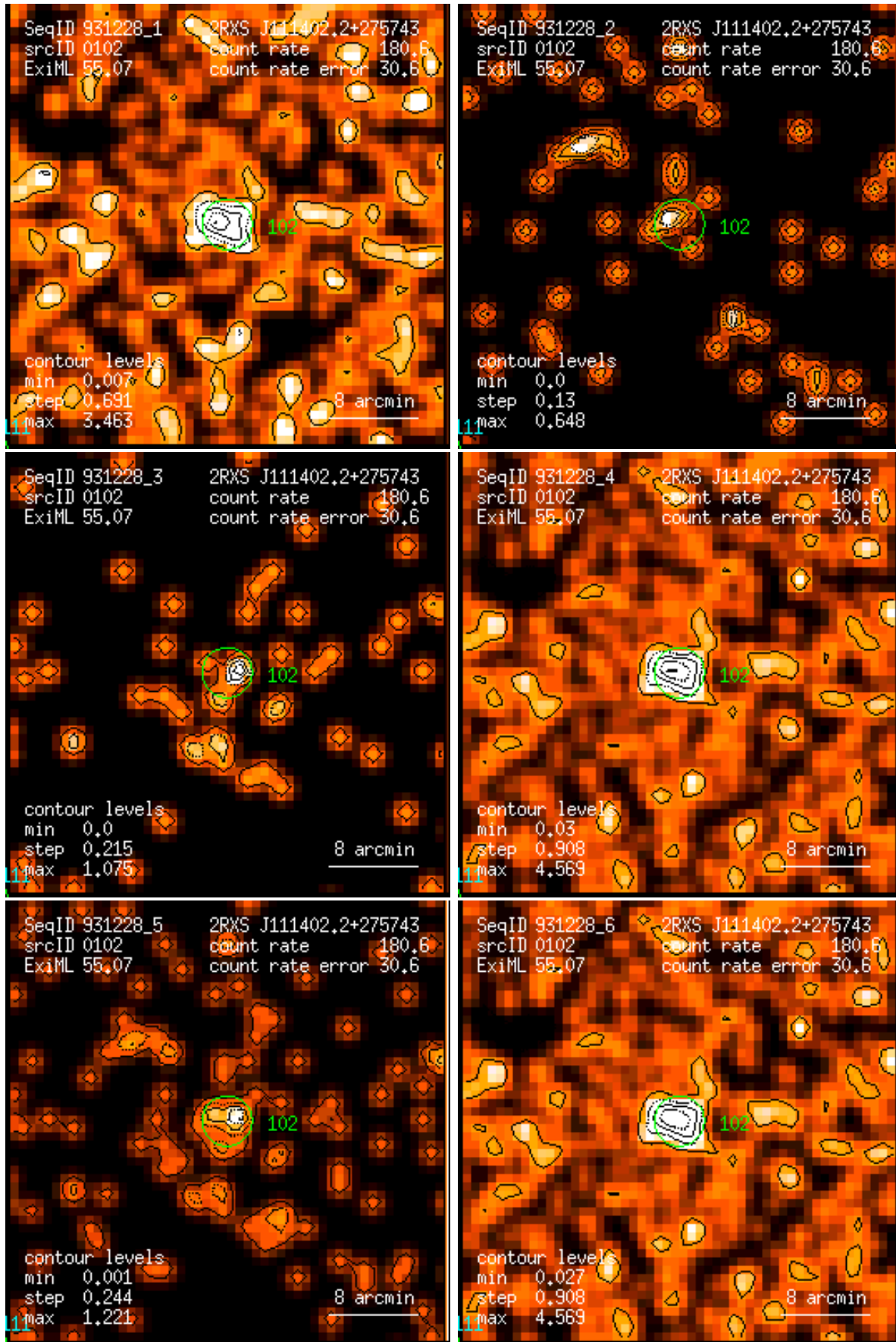
Figure 102: RASS 931228: detection 0102: band rate images, Gaussian filter: (1) PSPC channels 11 – 41, (2) 52 – 90, (3) 91 – 201, (4) 11 – 235, (5) 52 – 201, (6) 11 – 201. Broad band rates in counts/ks. Band rate contour levels in counts/ks/arcmin 2 .
