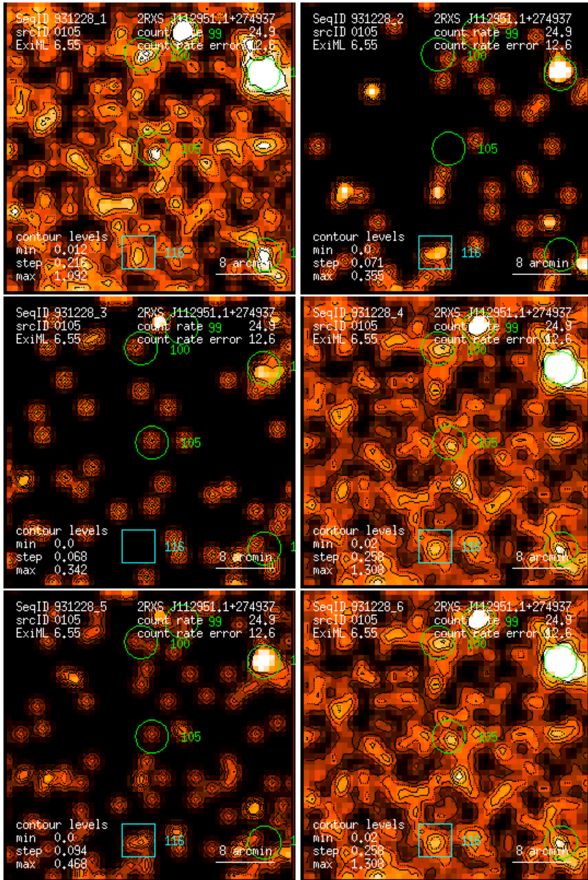
Figure 105: RASS 931228: detection 0105: band rate images, Gaussian filter: (1) PSPC channels 11 – 41, (2) 52 – 90, (3) 91 – 201, (4) 11 – 235, (5) 52 – 201, (6) 11 – 201. Broad band rates in counts/ks. Band rate contour levels in counts/ks/arcmin 2 .
