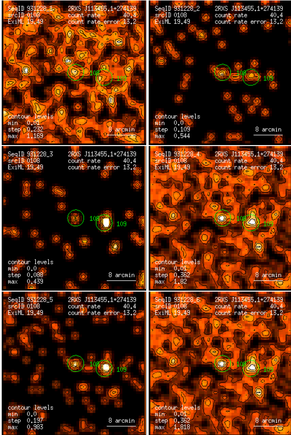
Figure 108: RASS 931228: detection 0108: band rate images, Gaussian filter: (1) PSPC channels 11 – 41, (2) 52 – 90, (3) 91 – 201, (4) 11 – 235, (5) 52 – 201, (6) 11 – 201. Broad band rates in counts/ks. Band rate contour levels in counts/ks/arcmin 2 .
