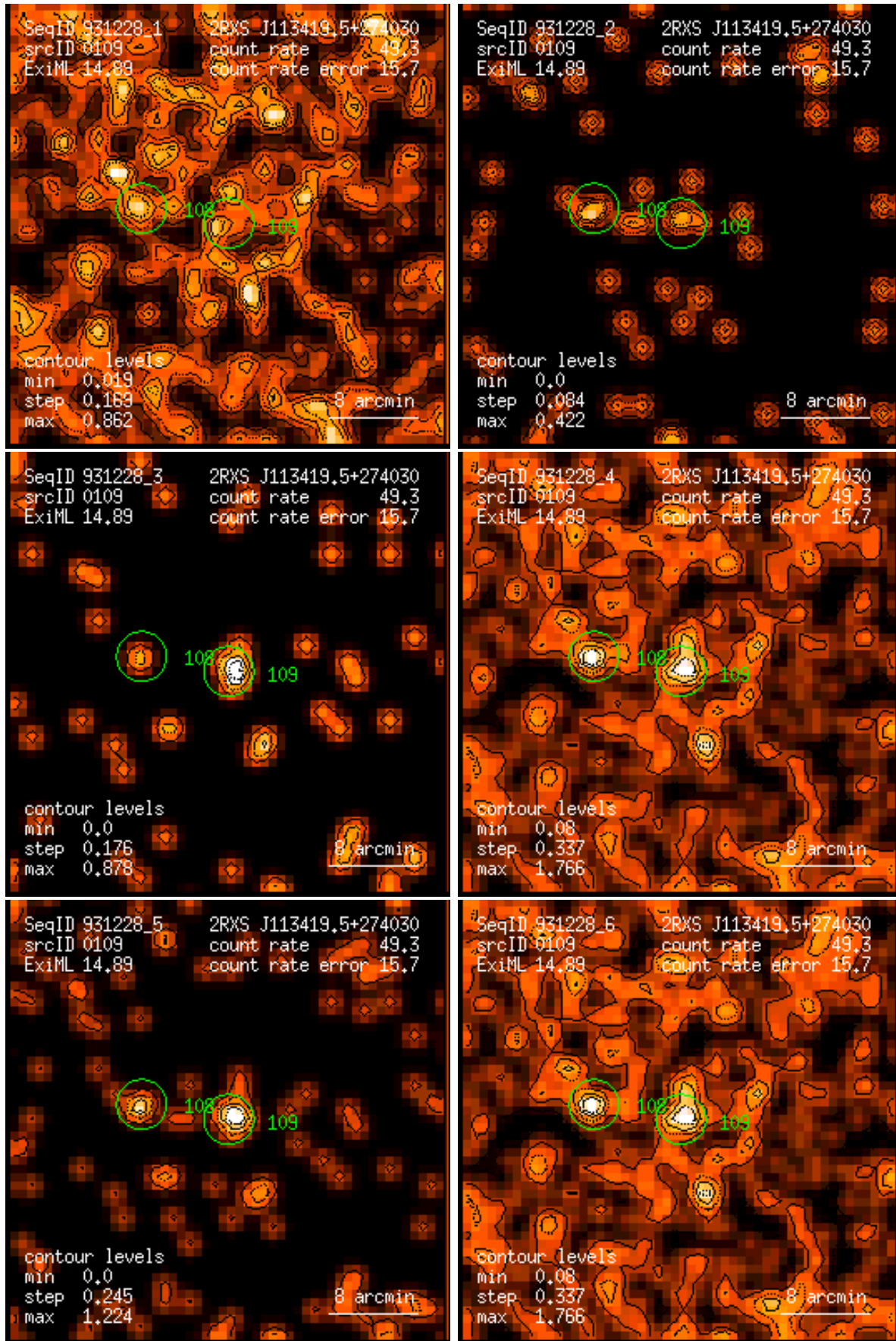
Figure 109: RASS 931228: detection 0109: band rate images, Gaussian filter: (1) PSPC channels 11 – 41, (2) 52 – 90, (3) 91 – 201, (4) 11 – 235, (5) 52 – 201, (6) 11 – 201. Broad band rates in counts/ks. Band rate contour levels in counts/ks/arcmin 2 .
