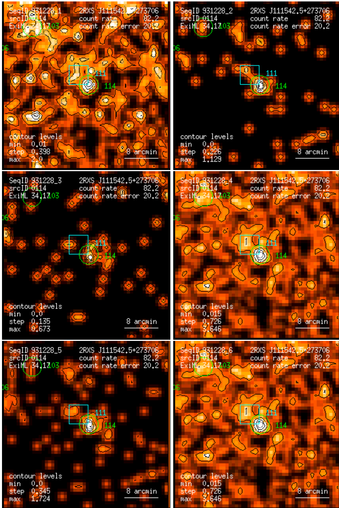
Figure 114: RASS 931228: detection 0114: band rate images, Gaussian filter: (1) PSPC channels 11 – 41, (2) 52 – 90, (3) 91 – 201, (4) 11 – 235, (5) 52 – 201, (6) 11 – 201. Broad band rates in counts/ks. Band rate contour levels in counts/ks/arcmin 2 .
