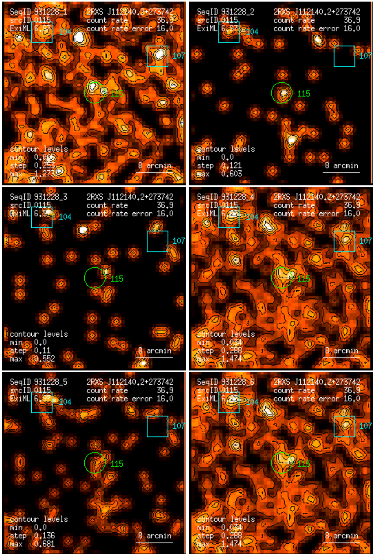
Figure 115: RASS 931228: detection 0115: band rate images, Gaussian filter: (1) PSPC channels 11 – 41, (2) 52 – 90, (3) 91 – 201, (4) 11 – 235, (5) 52 – 201, (6) 11 – 201. Broad band rates in counts/ks. Band rate contour levels in counts/ks/arcmin 2 .
