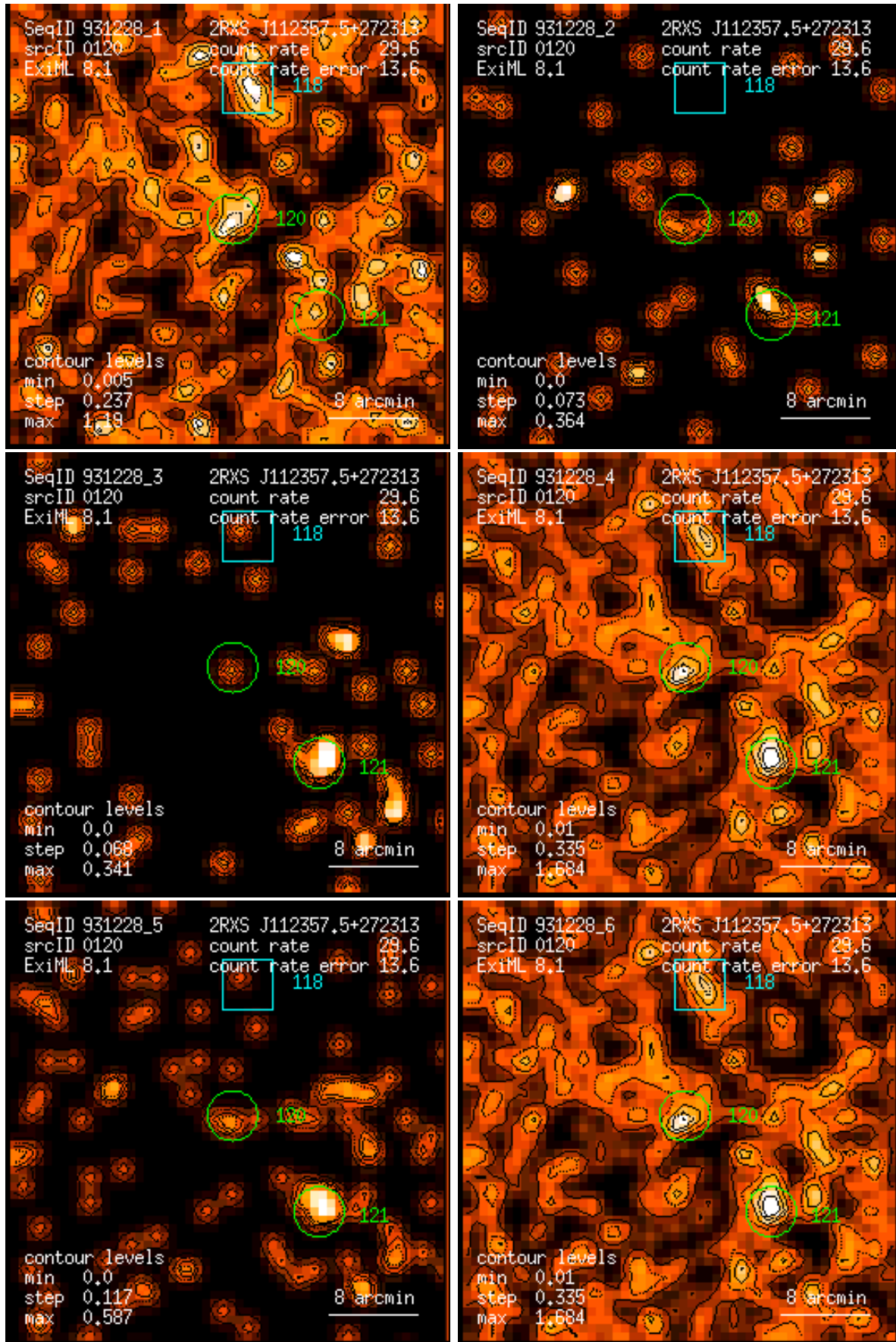
Figure 120: RASS 931228: detection 0120: band rate images, Gaussian filter: (1) PSPC channels 11 – 41, (2) 52 – 90, (3) 91 – 201, (4) 11 – 235, (5) 52 – 201, (6) 11 – 201. Broad band rates in counts/ks. Band rate contour levels in counts/ks/arcmin 2 .
