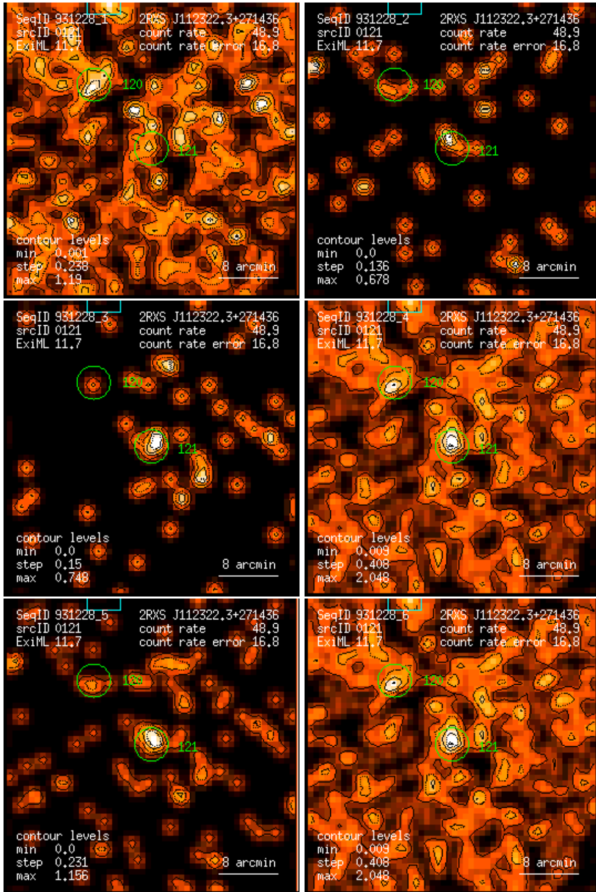
Figure 121: RASS 931228: detection 0121: band rate images, Gaussian filter: (1) PSPC channels 11 – 41, (2) 52 – 90, (3) 91 – 201, (4) 11 – 235, (5) 52 – 201, (6) 11 – 201. Broad band rates in counts/ks. Band rate contour levels in counts/ks/arcmin 2 .
