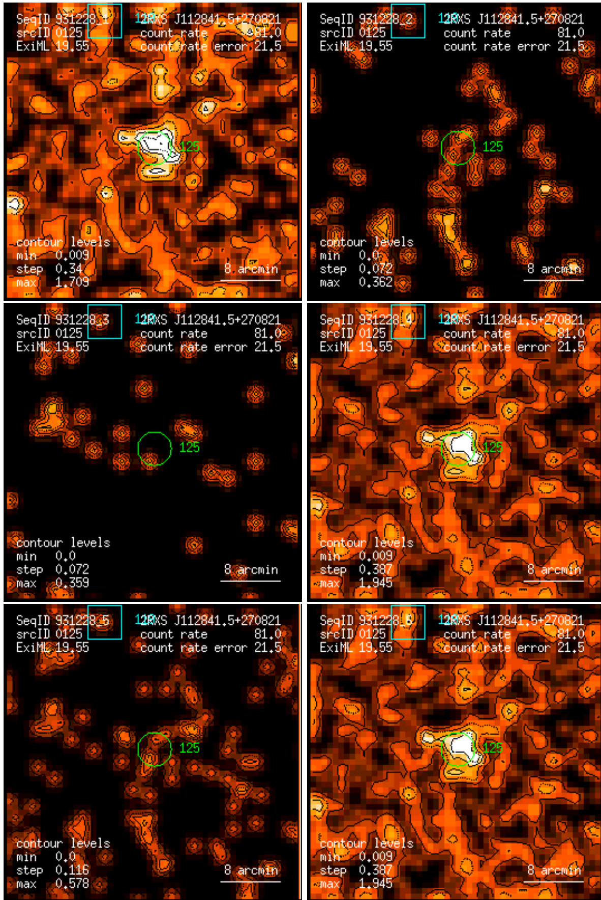
Figure 125: RASS 931228: detection 0125: band rate images, Gaussian filter: (1) PSPC channels 11 – 41, (2) 52 – 90, (3) 91 – 201, (4) 11 – 235, (5) 52 – 201, (6) 11 – 201. Broad band rates in counts/ks. Band rate contour levels in counts/ks/arcmin 2 .
