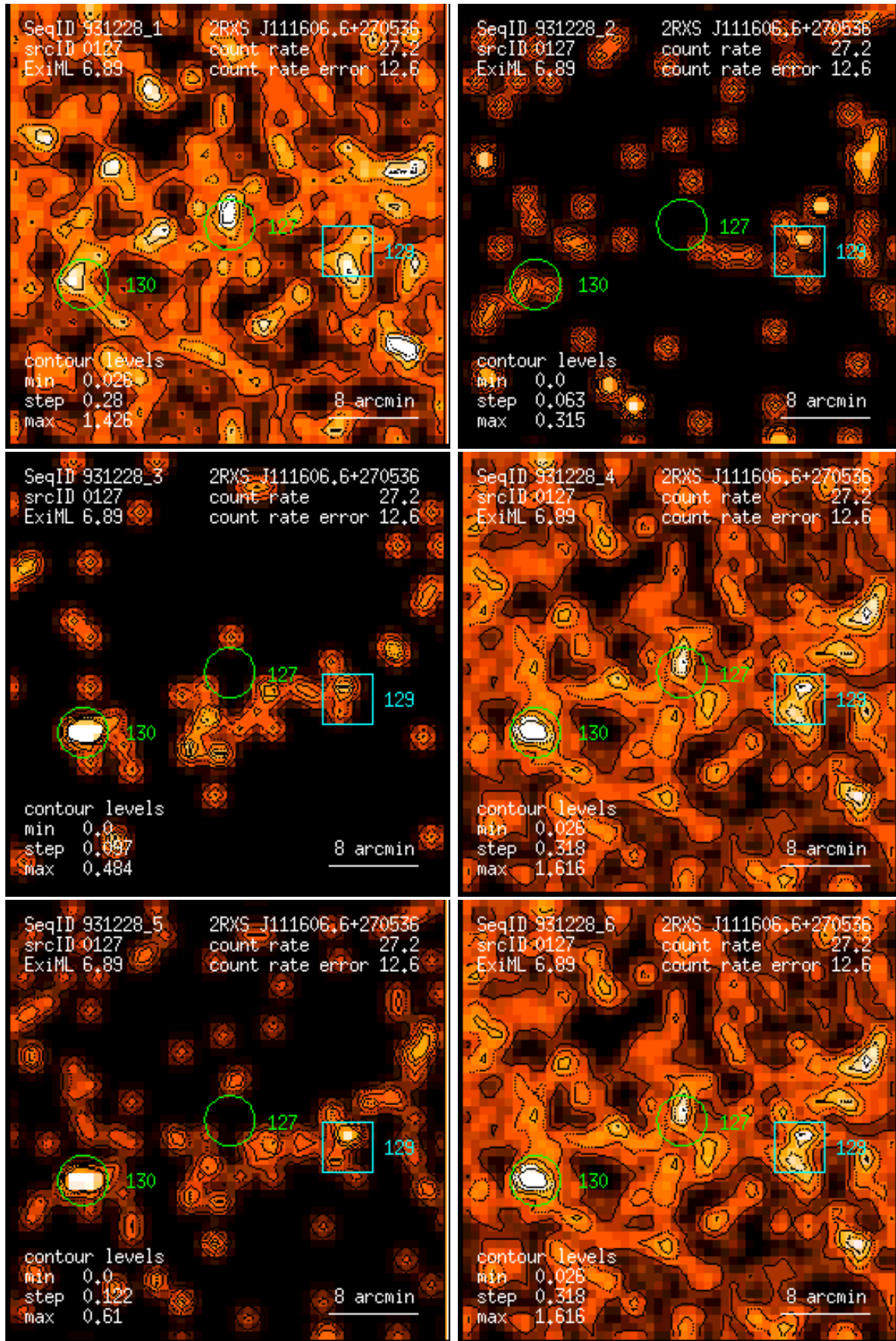
Figure 127: RASS 931228: detection 0127: band rate images, Gaussian filter: (1) PSPC channels 11 – 41, (2) 52 – 90, (3) 91 – 201, (4) 11 – 235, (5) 52 – 201, (6) 11 – 201. Broad band rates in counts/ks. Band rate contour levels in counts/ks/arcmin 2 .
