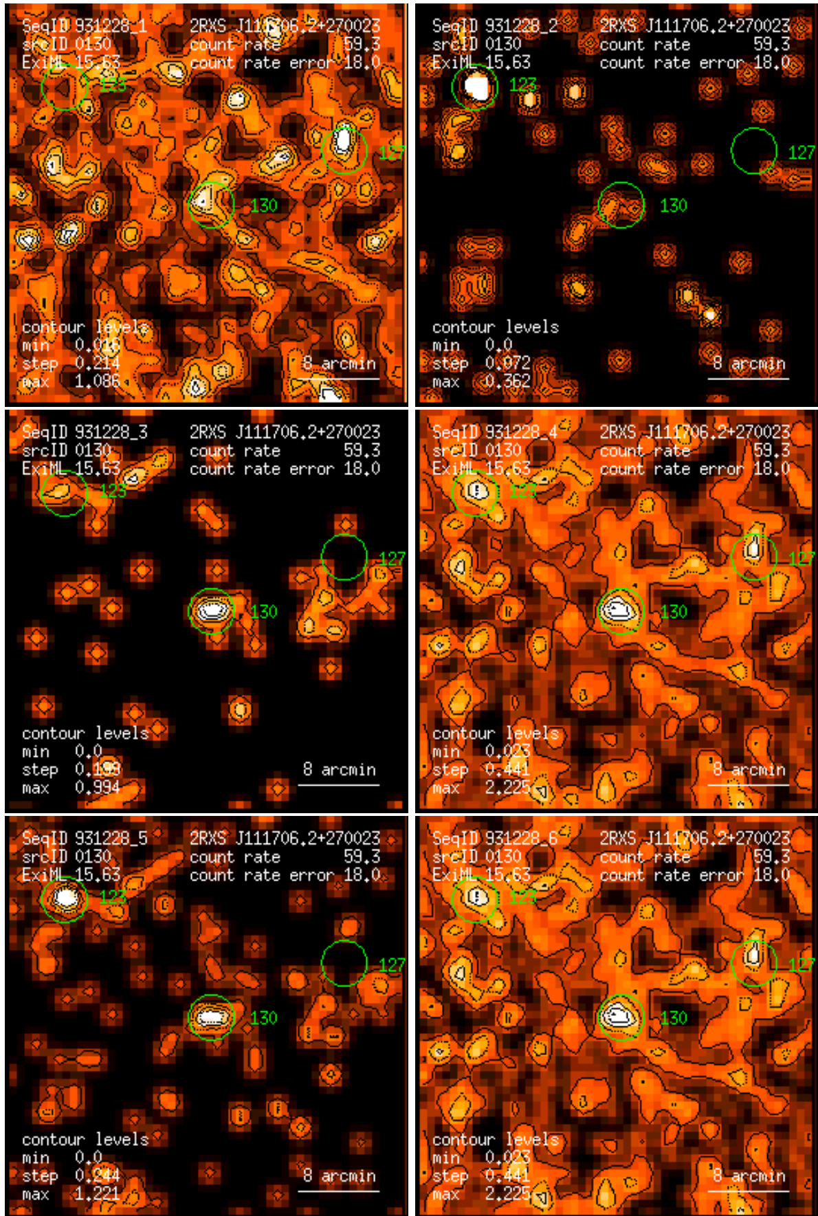
Figure 130: RASS 931228: detection 0130: band rate images, Gaussian filter: (1) PSPC channels 11 – 41, (2) 52 – 90, (3) 91 – 201, (4) 11 – 235, (5) 52 – 201, (6) 11 – 201. Broad band rates in counts/ks. Band rate contour levels in counts/ks/arcmin 2 .
