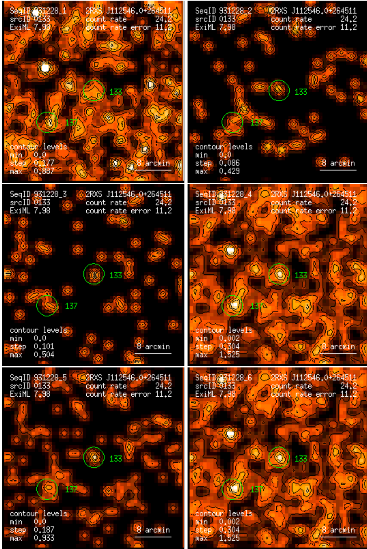
Figure 133: RASS 931228: detection 0133: band rate images, Gaussian filter: (1) PSPC channels 11 – 41, (2) 52 – 90, (3) 91 – 201, (4) 11 – 235, (5) 52 – 201, (6) 11 – 201. Broad band rates in counts/ks. Band rate contour levels in counts/ks/arcmin 2 .
