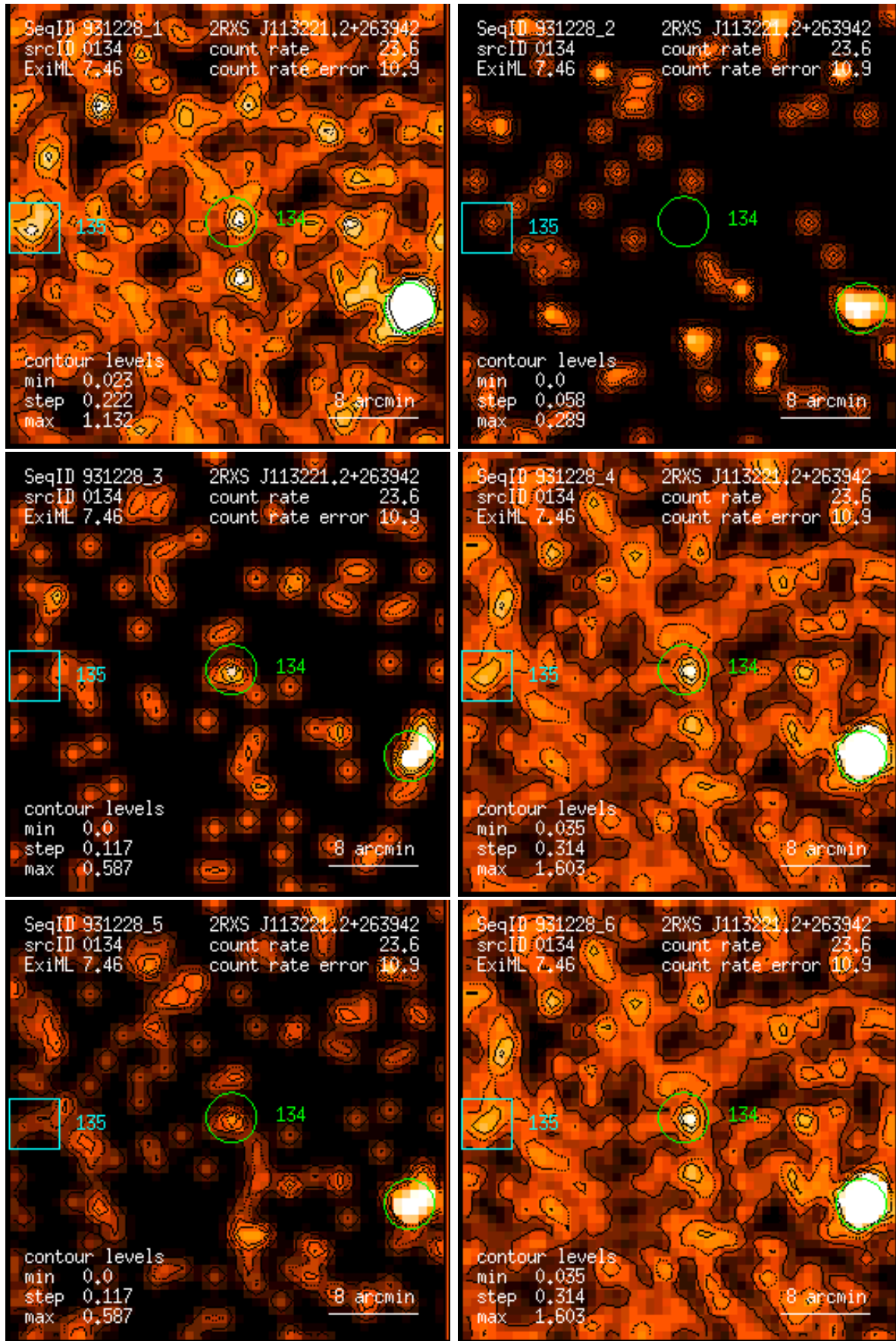
Figure 134: RASS 931228: detection 0134: band rate images, Gaussian filter: (1) PSPC channels 11 – 41, (2) 52 – 90, (3) 91 – 201, (4) 11 – 235, (5) 52 – 201, (6) 11 – 201. Broad band rates in counts/ks. Band rate contour levels in counts/ks/arcmin 2 .
