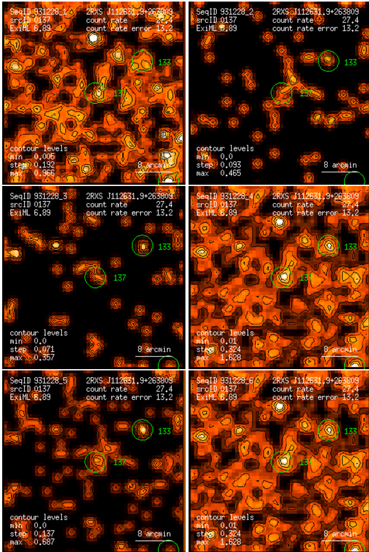
Figure 137: RASS 931228: detection 0137: band rate images, Gaussian filter: (1) PSPC channels 11 – 41, (2) 52 – 90, (3) 91 – 201, (4) 11 – 235, (5) 52 – 201, (6) 11 – 201. Broad band rates in counts/ks. Band rate contour levels in counts/ks/arcmin 2 .
