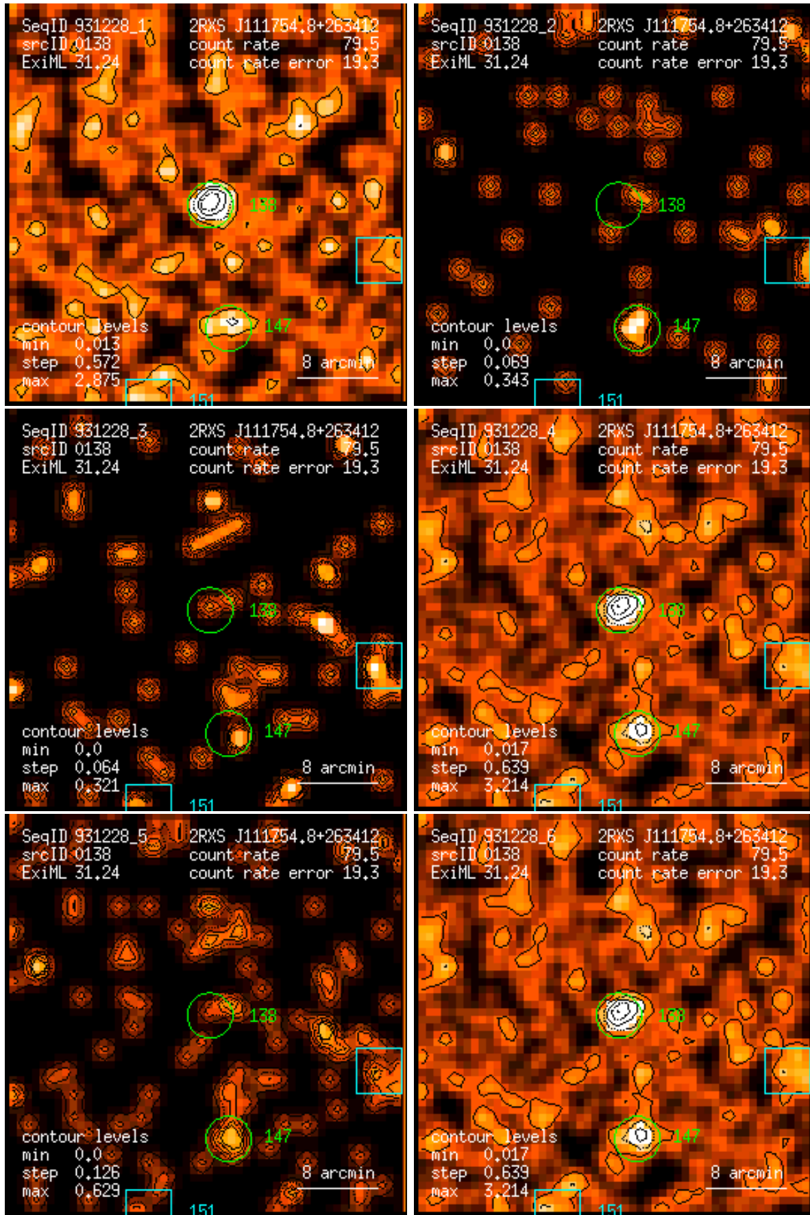
Figure 138: RASS 931228: detection 0138: band rate images, Gaussian filter: (1) PSPC channels 11 – 41, (2) 52 – 90, (3) 91 – 201, (4) 11 – 235, (5) 52 – 201, (6) 11 – 201. Broad band rates in counts/ks. Band rate contour levels in counts/ks/arcmin 2 .
