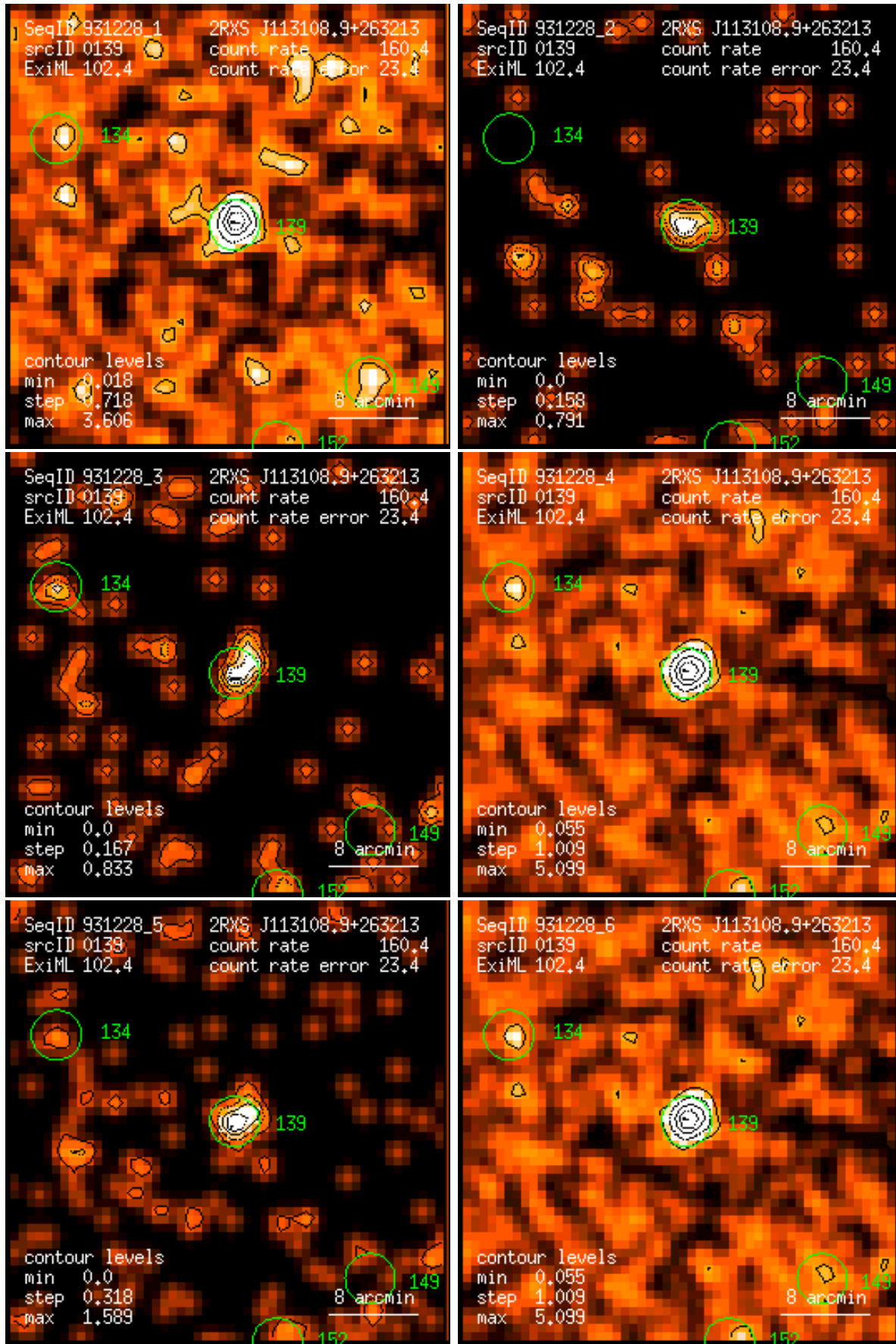
Figure 139: RASS 931228: detection 0139: band rate images, Gaussian filter: (1) PSPPC channels 11 – 41, (2) 52 – 90, (3) 91 – 201, (4) 11 – 235, (5) 52 – 201, (6) 11 – 201. Broad band rates in counts/ks. Band rate contour levels in counts/ks/arcmin 2 .
