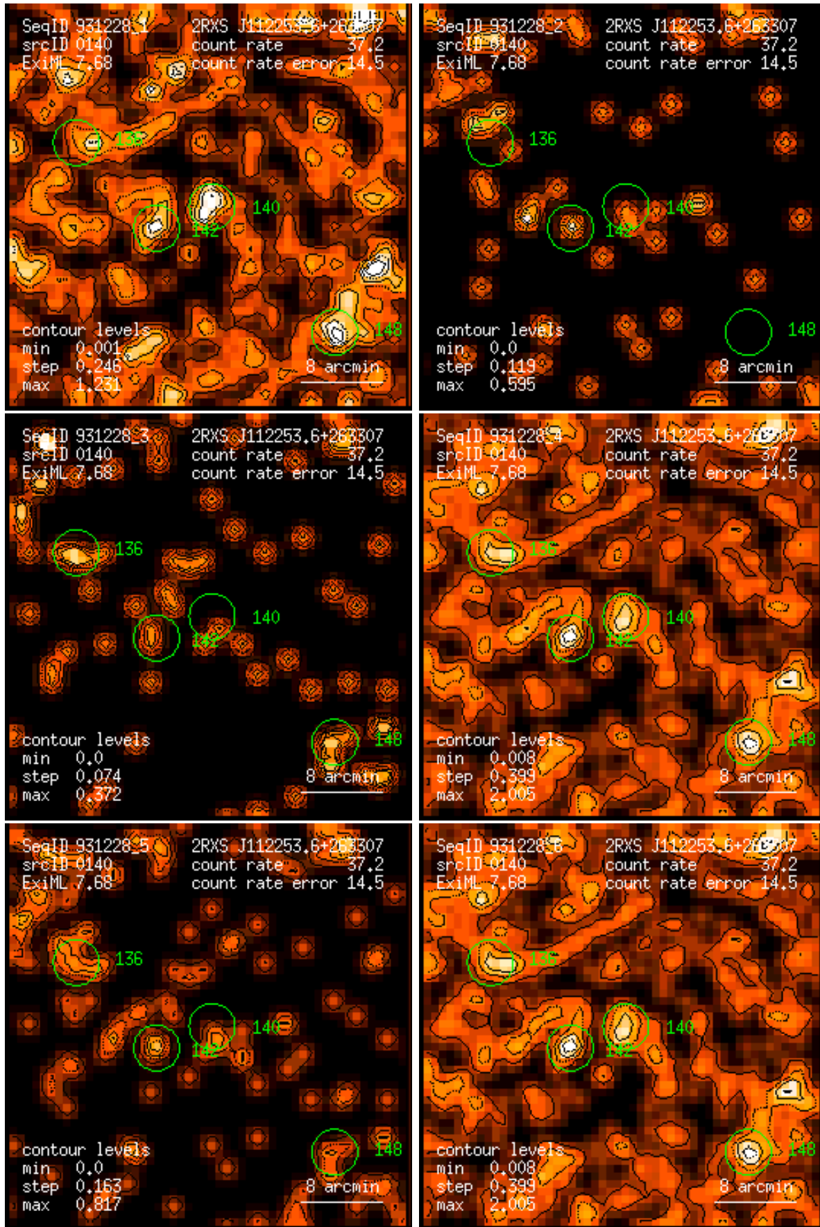
Figure 140: RASS 931228: detection 0140: band rate images, Gaussian filter: (1) PSPC channels 11 – 41, (2) 52 – 90, (3) 91 – 201, (4) 11 – 235, (5) 52 – 201, (6) 11 – 201. Broad band rates in counts/ks. Band rate contour levels in counts/ks/arcmin 2 .
