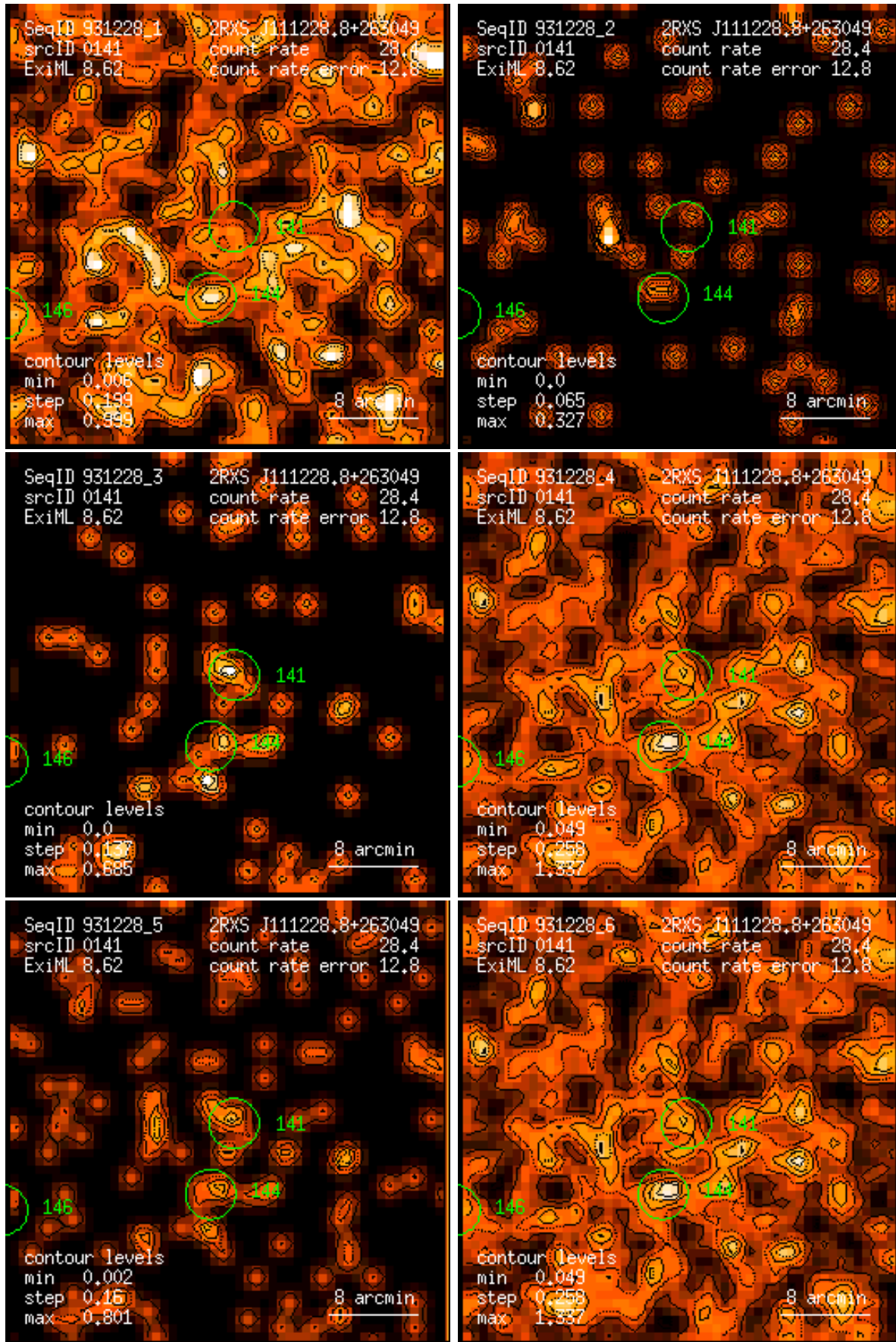
Figure 141: RASS 931228: detection 0141: band rate images, Gaussian filter: (1) PSPC channels 11 – 41, (2) 52 – 90, (3) 91 – 201, (4) 11 – 235, (5) 52 – 201, (6) 11 – 201. Broad band rates in counts/ks. Band rate contour levels in counts/ks/arcmin 2 .
