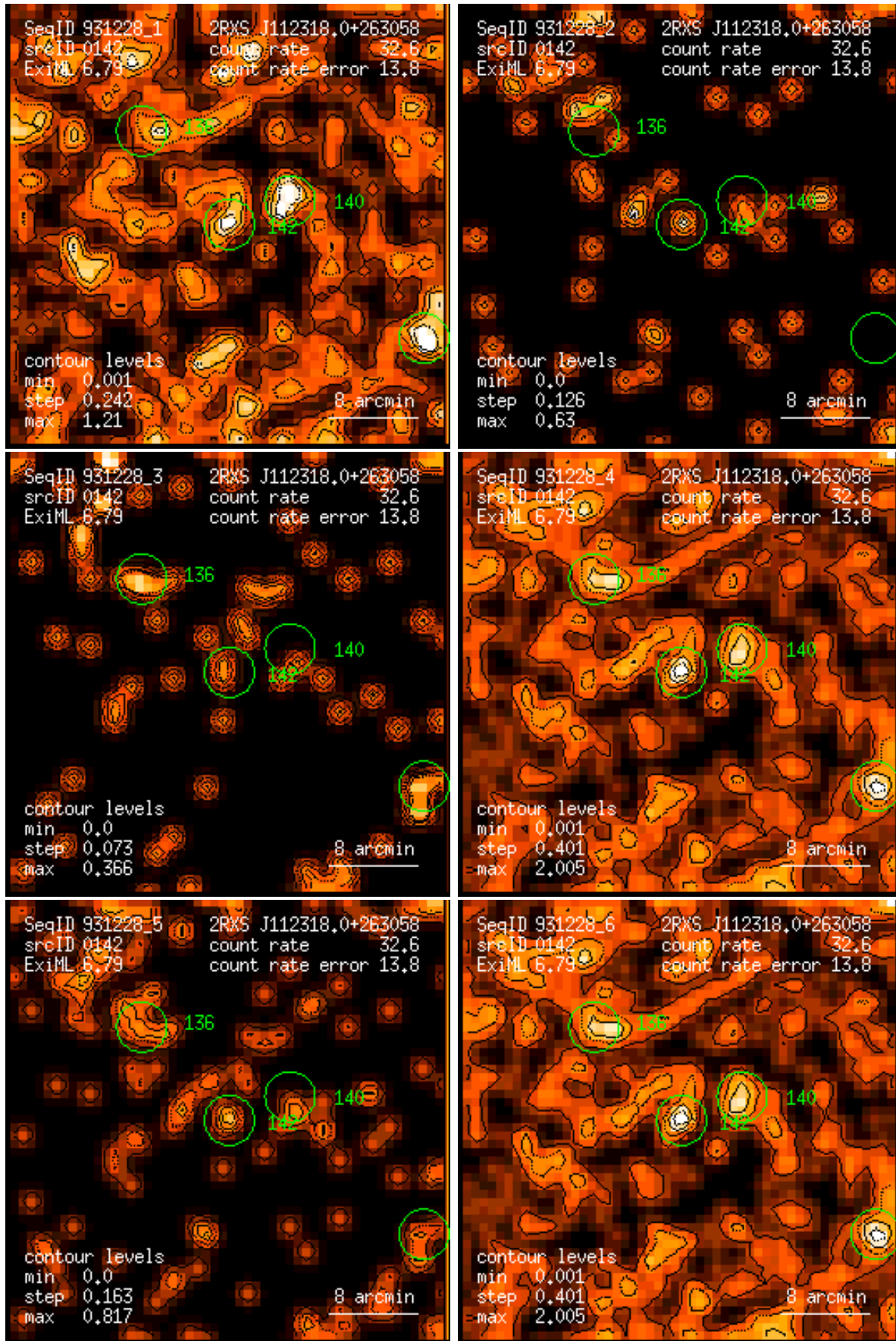
Figure 142: RASS 931228: detection 0142: band rate images, Gaussian filter: (1) PSPC channels 11 – 41, (2) 52 – 90, (3) 91 – 201, (4) 11 – 235, (5) 52 – 201, (6) 11 – 201. Broad band rates in counts/ks. Band rate contour levels in counts/ks/arcmin 2 .
