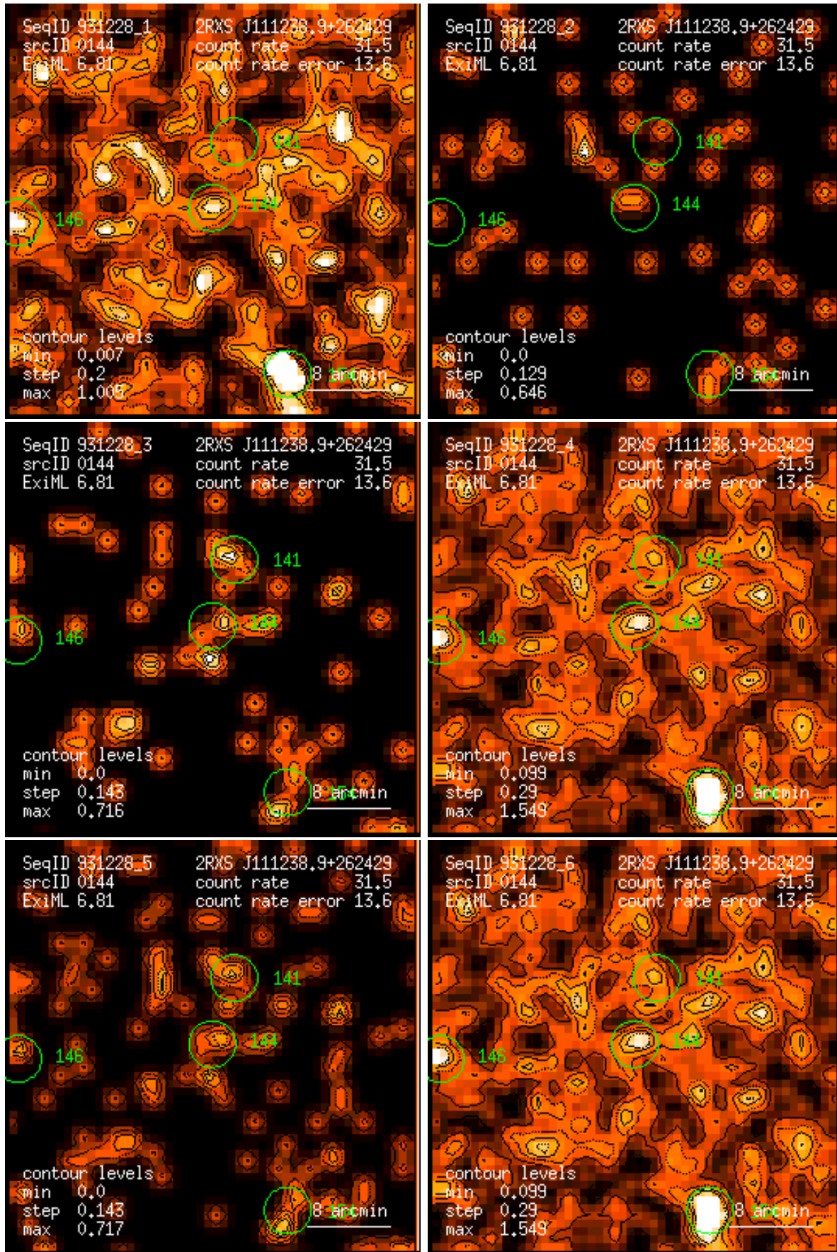
Figure 144: RASS 931228: detection 0144: band rate images, Gaussian filter: (1) PSPC channels 11 – 41, (2) 52 – 90, (3) 91 – 201, (4) 11 – 235, (5) 52 – 201, (6) 11 – 201. Broad band rates in counts/ks. Band rate contour levels in counts/ks/arcmin 2 .
