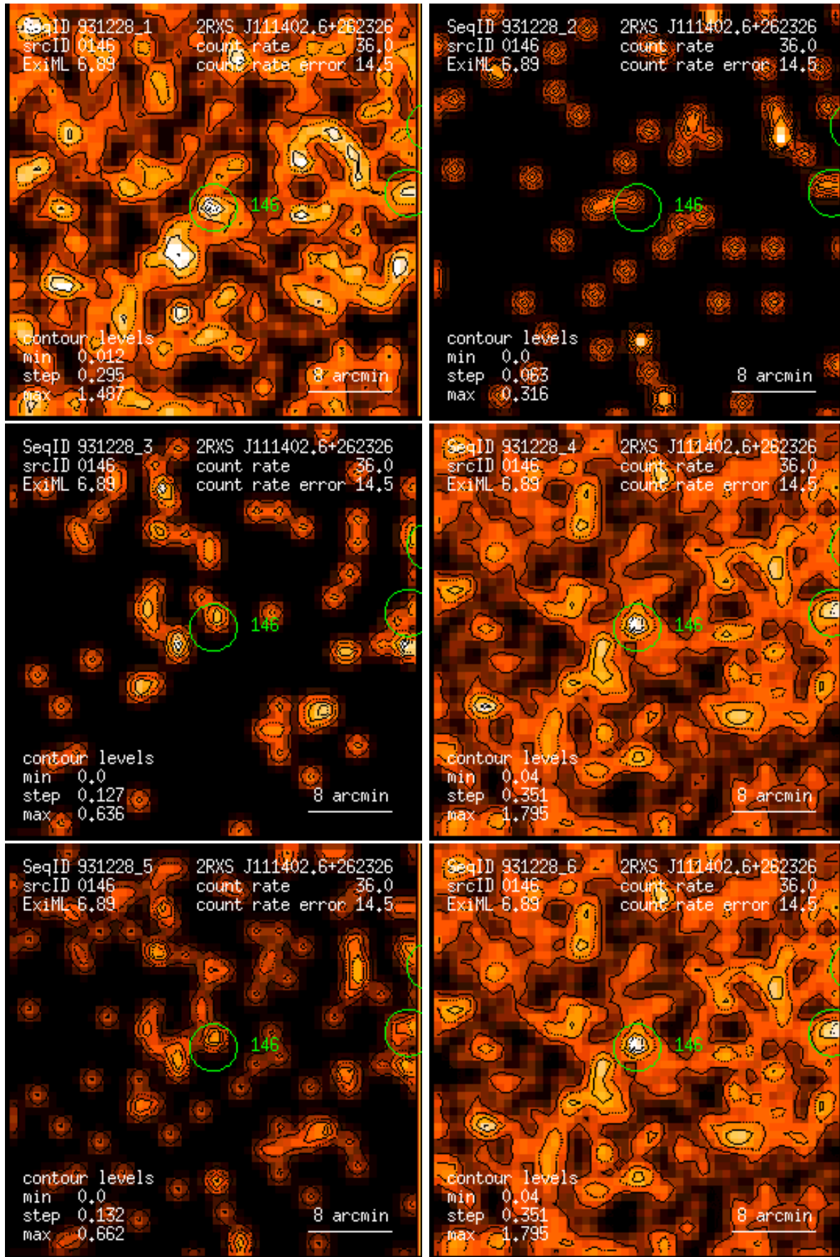
Figure 146: RASS 931228: detection 0146: band rate images, Gaussian filter: (1) PSPC channels 11 – 41, (2) 52 – 90, (3) 91 – 201, (4) 11 – 235, (5) 52 – 201, (6) 11 – 201. Broad band rates in counts/ks. Band rate contour levels in counts/ks/arcmin 2 .
