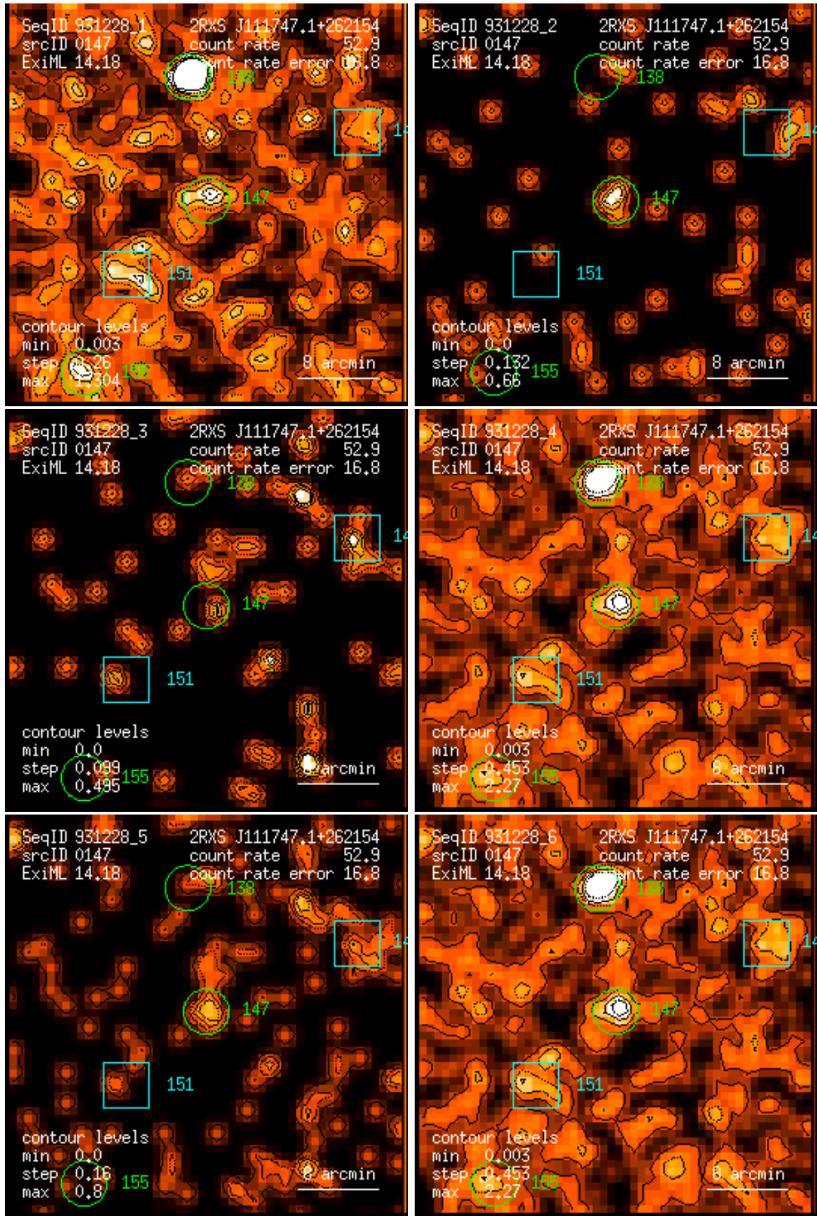
Figure 147: RASS 931228: detection 0147: band rate images, Gaussian filter: (1) PSPC channels 11 – 41, (2) 52 – 90, (3) 91 – 201, (4) 11 – 235, (5) 52 – 201, (6) 11 – 201. Broad band rates in counts/ks. Band rate contour levels in counts/ks/arcmin 2 .
