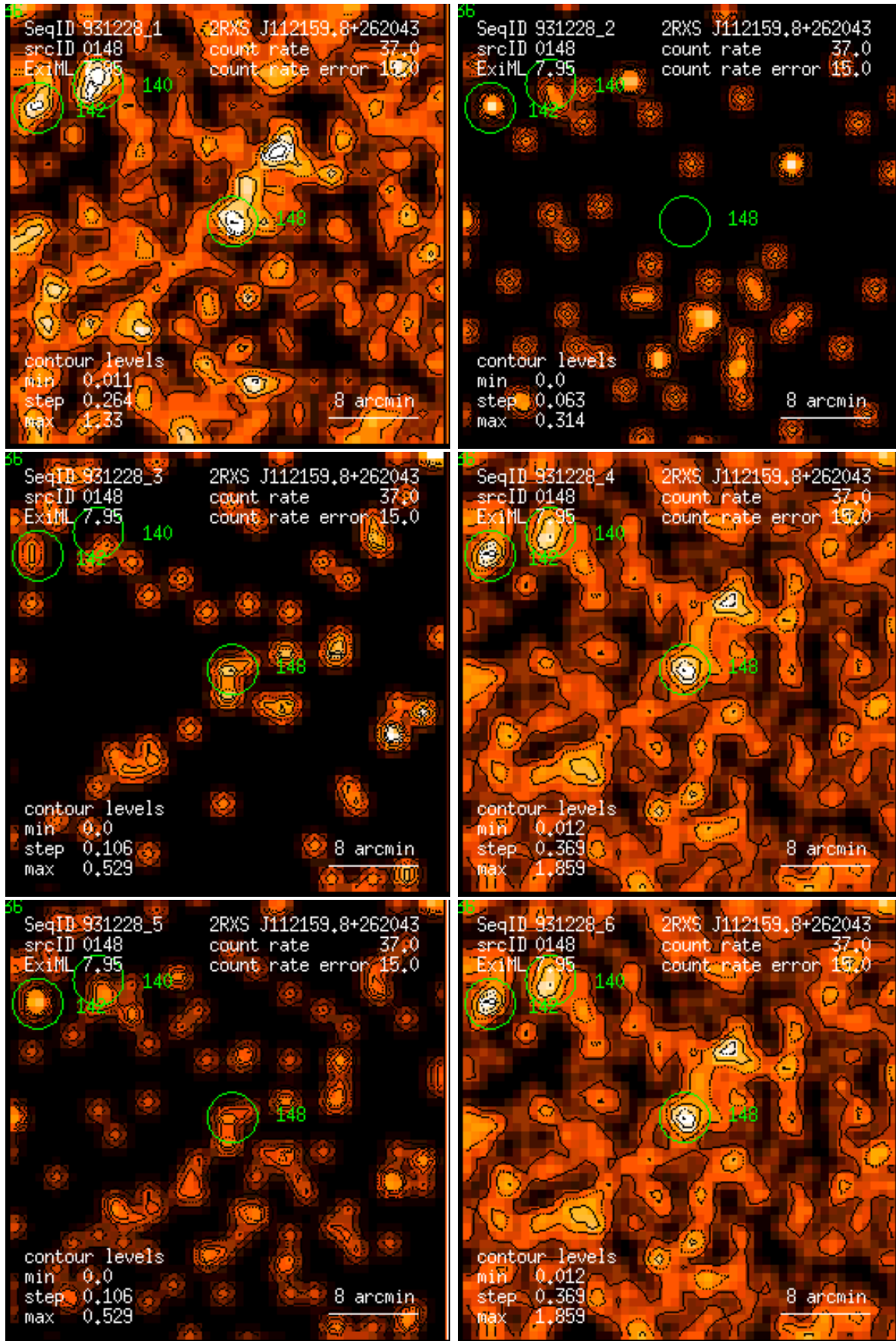
Figure 148: RASS 931228: detection 0148: band rate images, Gaussian filter: (1) PSPC channels 11 – 41, (2) 52 – 90, (3) 91 – 201, (4) 11 – 235, (5) 52 – 201, (6) 11 – 201. Broad band rates in counts/ks. Band rate contour levels in counts/ks/arcmin 2 .
