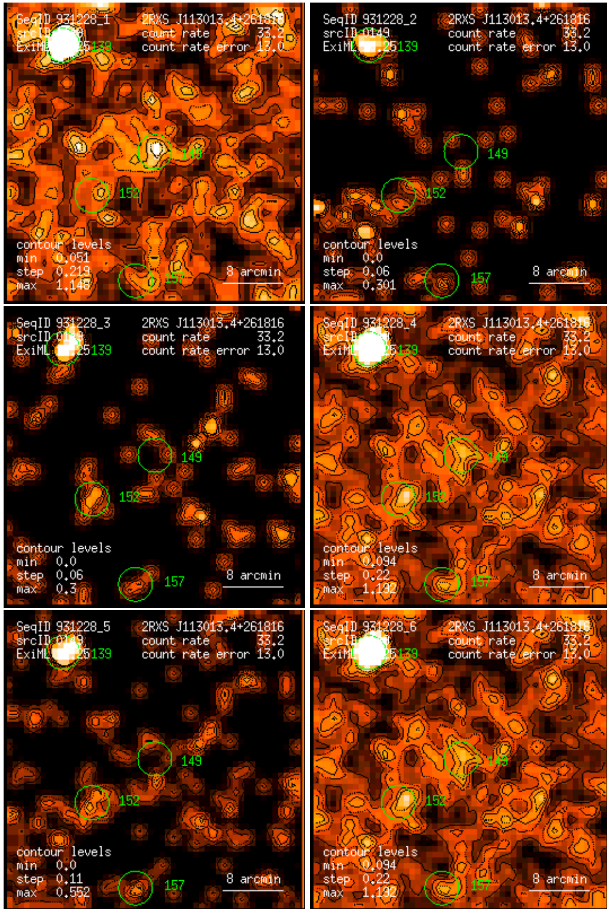
Figure 149: RASS 931228: detection 0149: band rate images, Gaussian filter: (1) PSPC channels 11 – 41, (2) 52 – 90, (3) 91 – 201, (4) 11 – 235, (5) 52 – 201, (6) 11 – 201. Broad band rates in counts/ks. Band rate contour levels in counts/ks/arcmin 2 .
