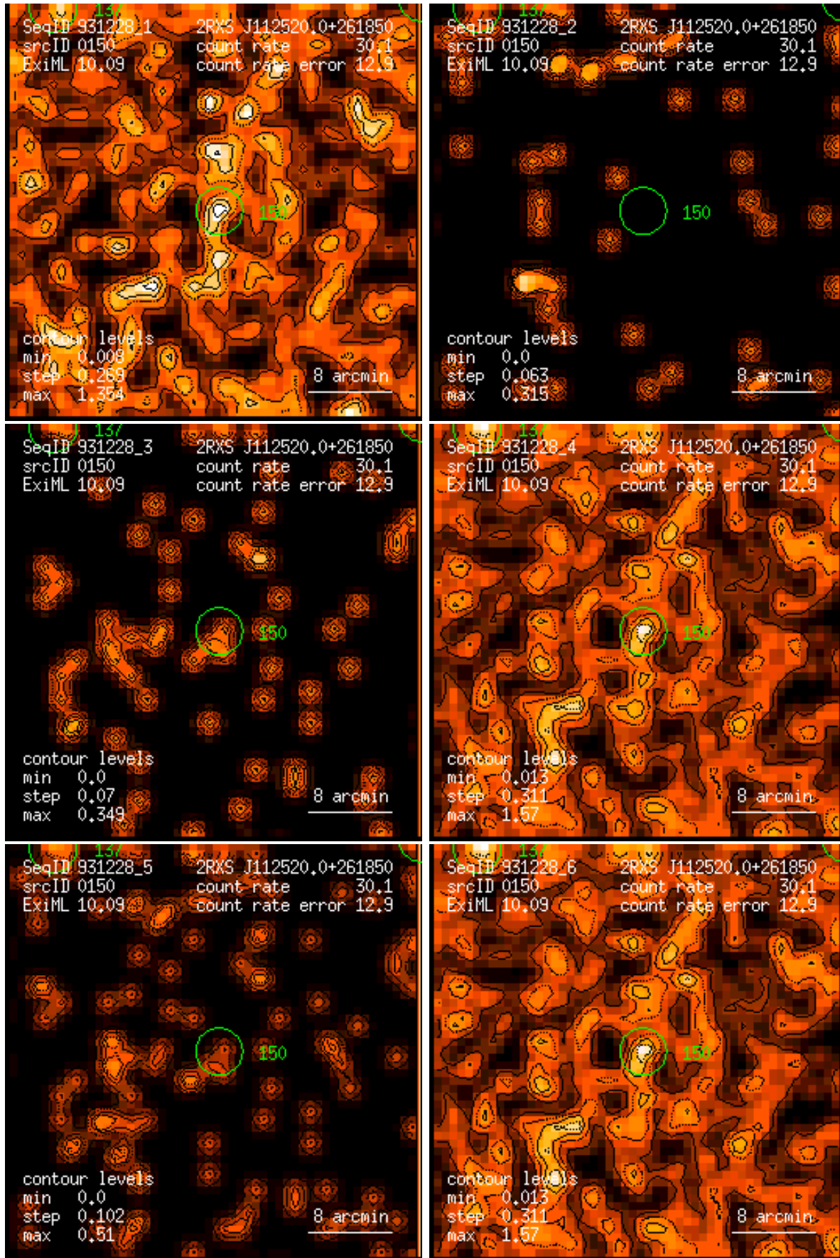
Figure 150: RASS 931228: detection 0150: band rate images, Gaussian filter: (1) PSPC channels 11 – 41, (2) 52 – 90, (3) 91 – 201, (4) 11 – 235, (5) 52 – 201, (6) 11 – 201. Broad band rates in counts/ks. Band rate contour levels in counts/ks/arcmin 2 .
