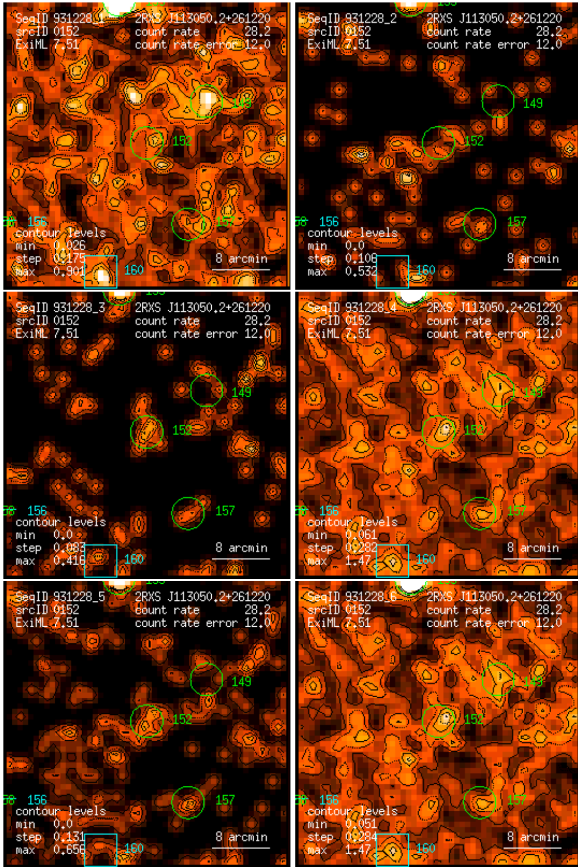
Figure 152: RASS 931228: detection 0152: band rate images, Gaussian filter: (1) PSPC channels 11 – 41, (2) 52 – 90, (3) 91 – 201, (4) 11 – 235, (5) 52 – 201, (6) 11 – 201. Broad band rates in counts/ks. Band rate contour levels in counts/ks/arcmin 2 .
