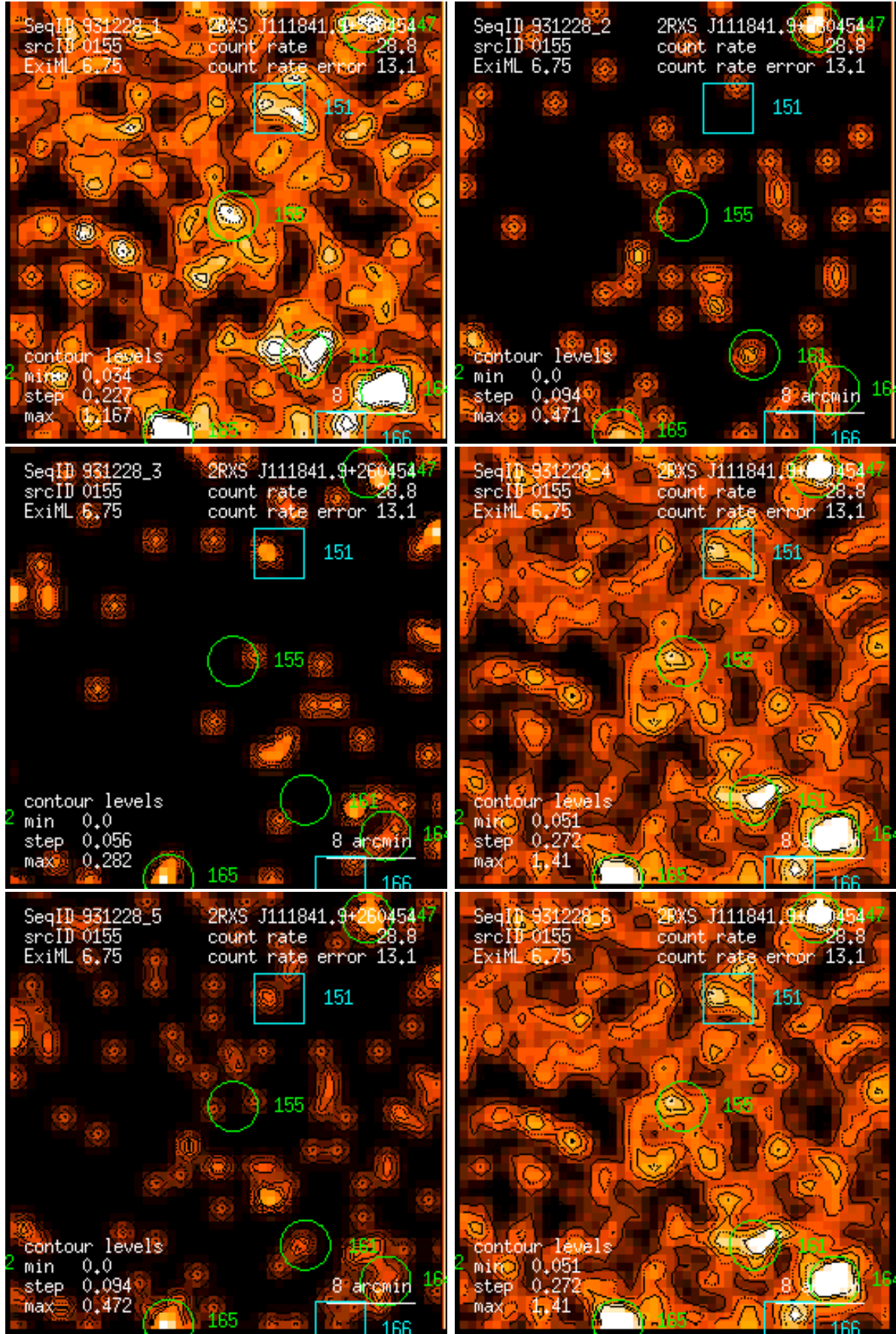
Figure 155: RASS 931228: detection 0155: band rate images, Gaussian filter: (1) PSPC channels 11 – 41, (2) 52 – 90, (3) 91 – 201, (4) 11 – 235, (5) 52 – 201, (6) 11 – 201. Broad band rates in counts/ks. Band rate contour levels in counts/ks/arcmin 2 .
