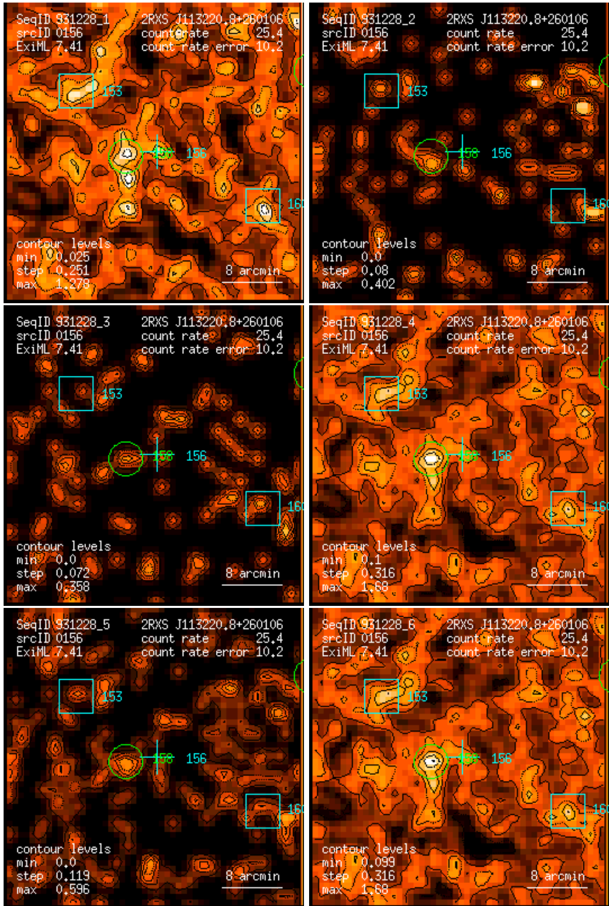
Figure 156: RASS 931228: detection 0156: band rate images, Gaussian filter: (1) PSPC channels 11 – 41, (2) 52 – 90, (3) 91 – 201, (4) 11 – 235, (5) 52 – 201, (6) 11 – 201. Broad band rates in counts/ks. Band rate contour levels in counts/ks/arcmin 2 .
