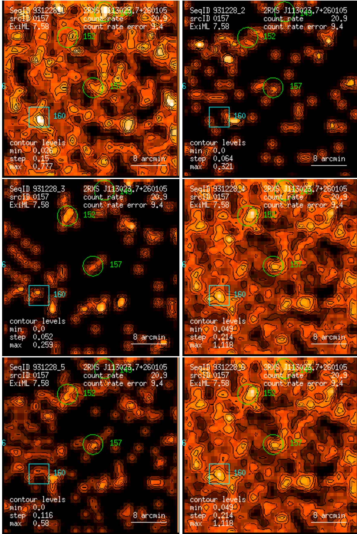
Figure 157: RASS 931228: detection 0157: band rate images, Gaussian filter: (1) PSPC channels 11 – 41, (2) 52 – 90, (3) 91 – 201, (4) 11 – 235, (5) 52 – 201, (6) 11 – 201. Broad band rates in counts/ks. Band rate contour levels in counts/ks/arcmin 2 .
