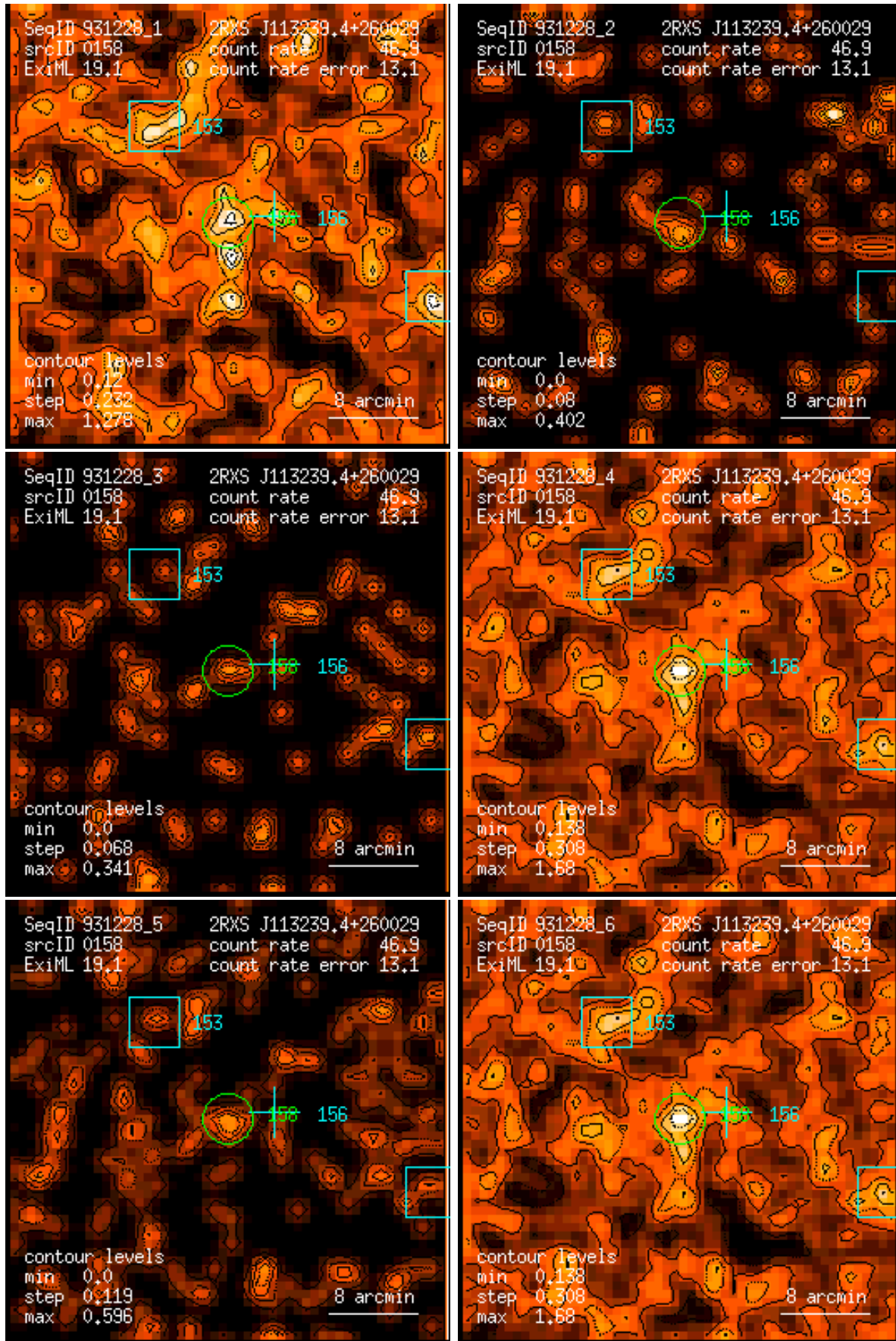
Figure 158: RASS 931228: detection 0158: band rate images, Gaussian filter: (1) PSPC channels 11 – 41, (2) 52 – 90, (3) 91 – 201, (4) 11 – 235, (5) 52 – 201, (6) 11 – 201. Broad band rates in counts/ks. Band rate contour levels in counts/ks/arcmin 2 .
